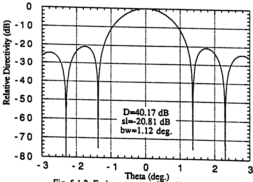
Fig. 5.1.2 E plane pattern of Design C, scan=0 deg.
