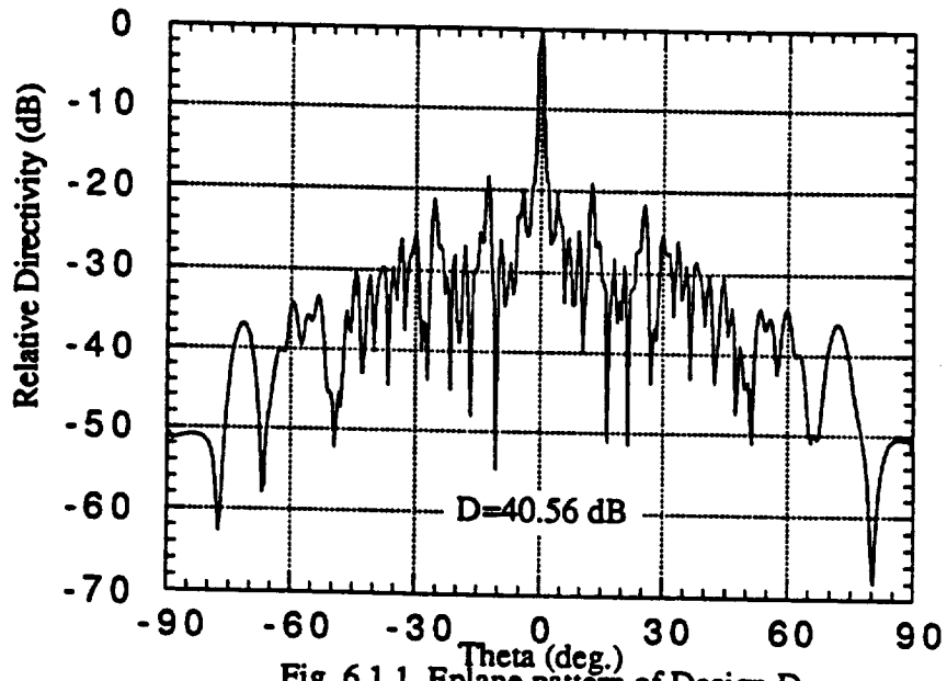
Fig. 6.1.1 Eplane pattern of Design D
