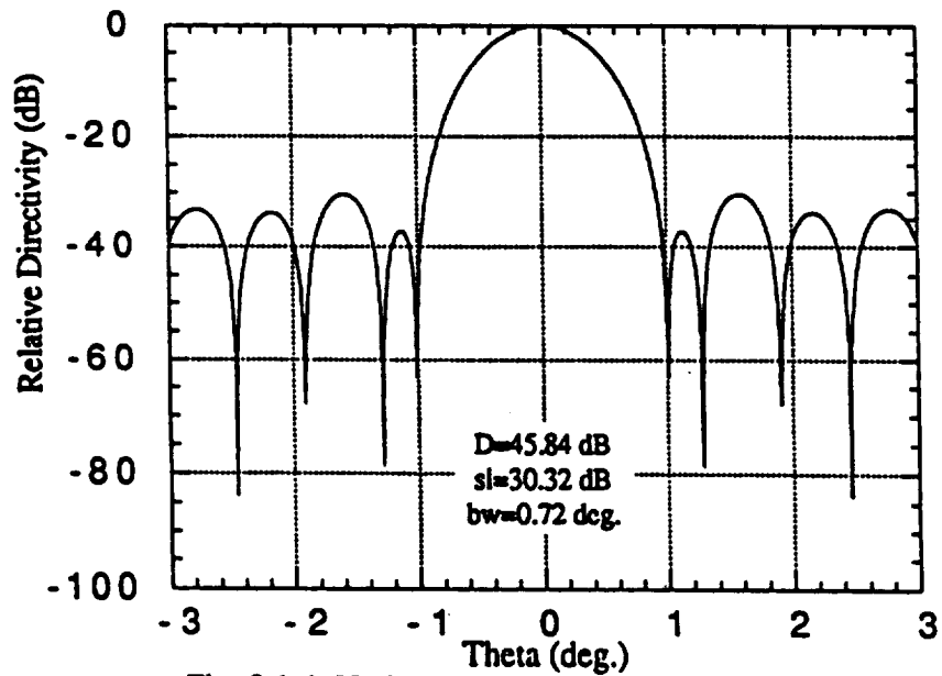
Fig. 3.1.4 H plane pattern of Design A1. scan=0 deg.
