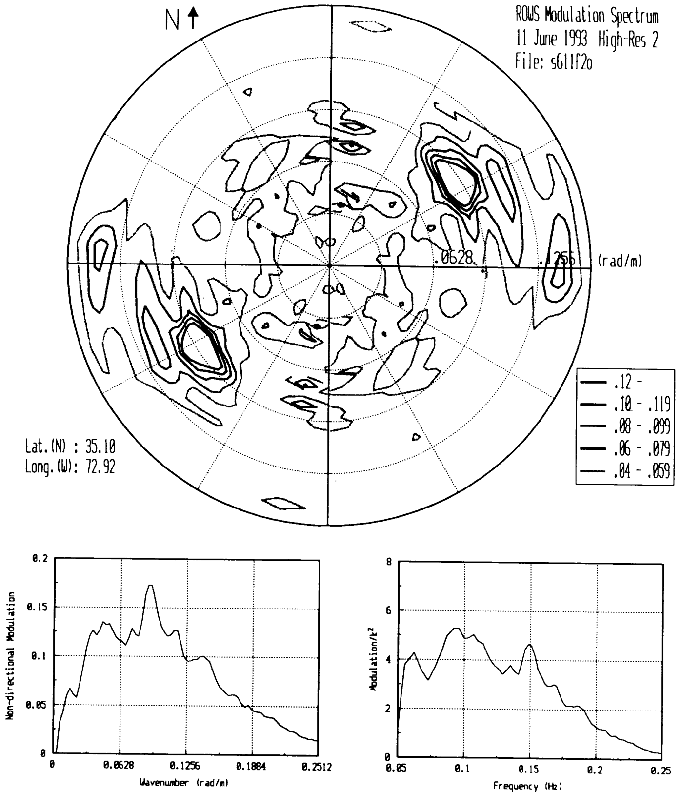
Figure 46. ROWS spectral data, file s611f2o.
