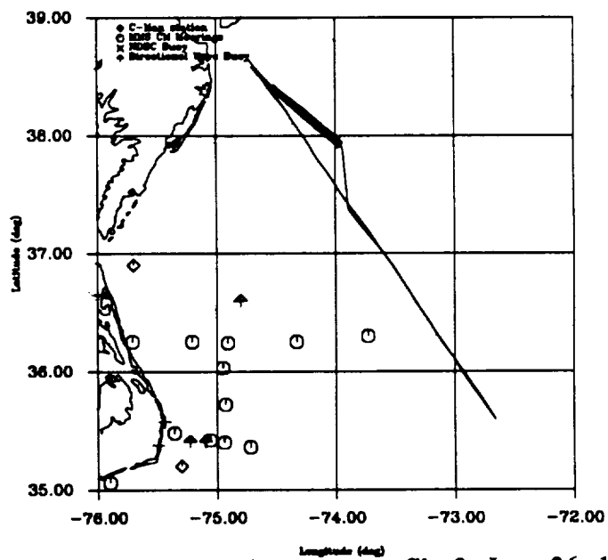
Figure 29. Altimeter mode summary, file 2, June 26, 1993.
