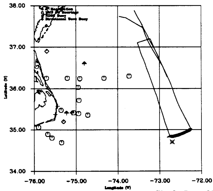
Figure 33. Altimeter mode summary, file 3, June 27, 1993.
