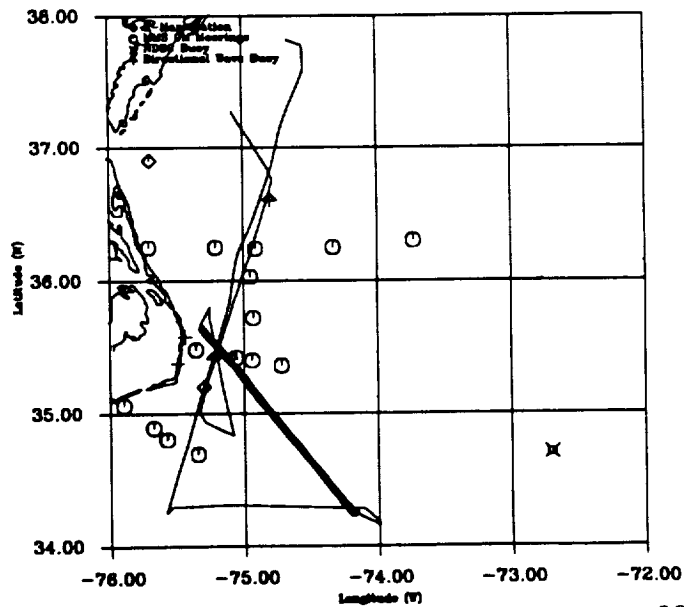
Figure 25. Altimeter mode summary, file 5, June 20, 1993.
