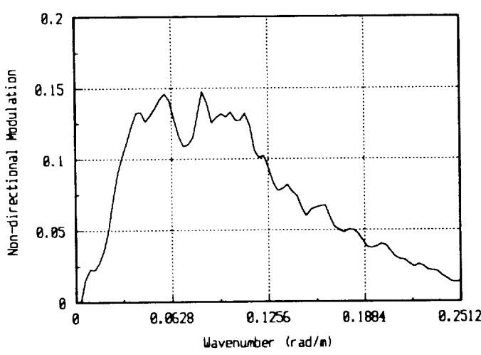
Figure 51. ROWS spectral data, file s614f8h.
