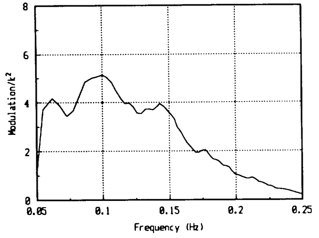
Figure 45. ROWS spectral data, file s611f2m.
