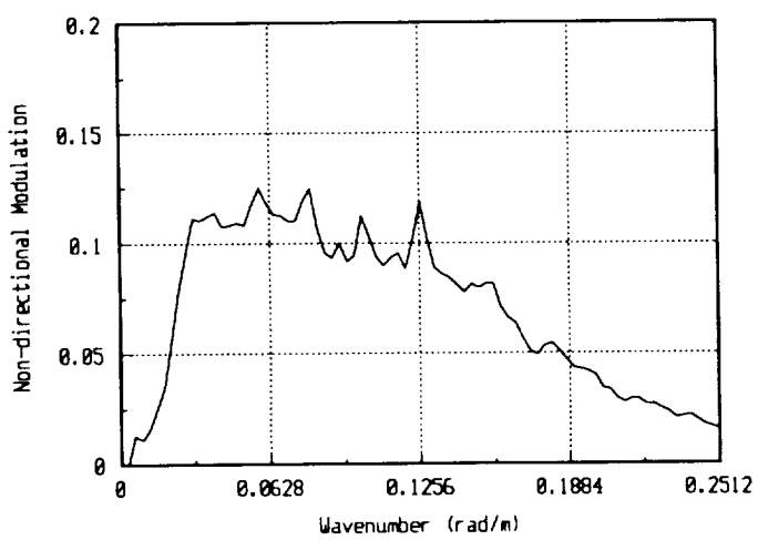
Figure 57. ROWS spectral data, file s626f4f.
