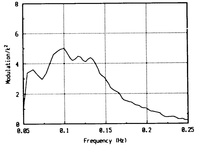
Figure 43. ROWS spectral data, file s611f2i.
