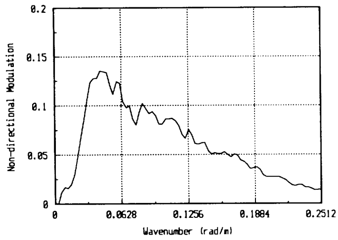
Figure 49. ROWS spectral data, file s614f30.
