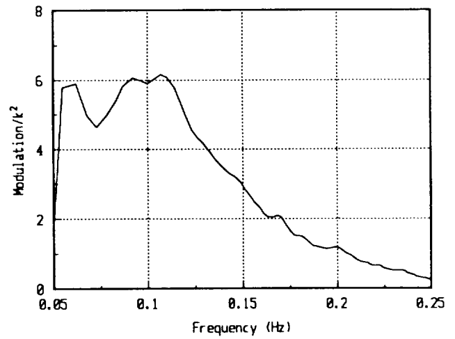
Figure 55. ROWS spectral data, file s620f2y.
