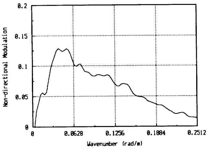
Figure 39. ROWS spectral data, file s611f2a.
