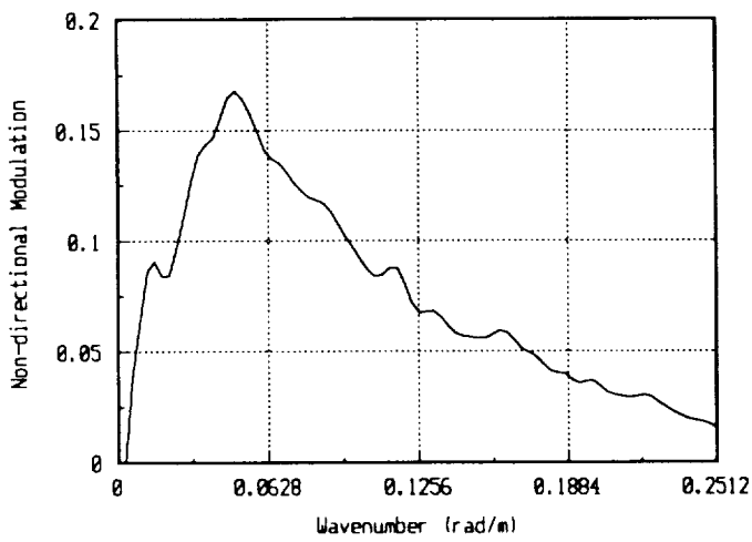
Figure 55. ROWS spectral data, file s620f2y.
