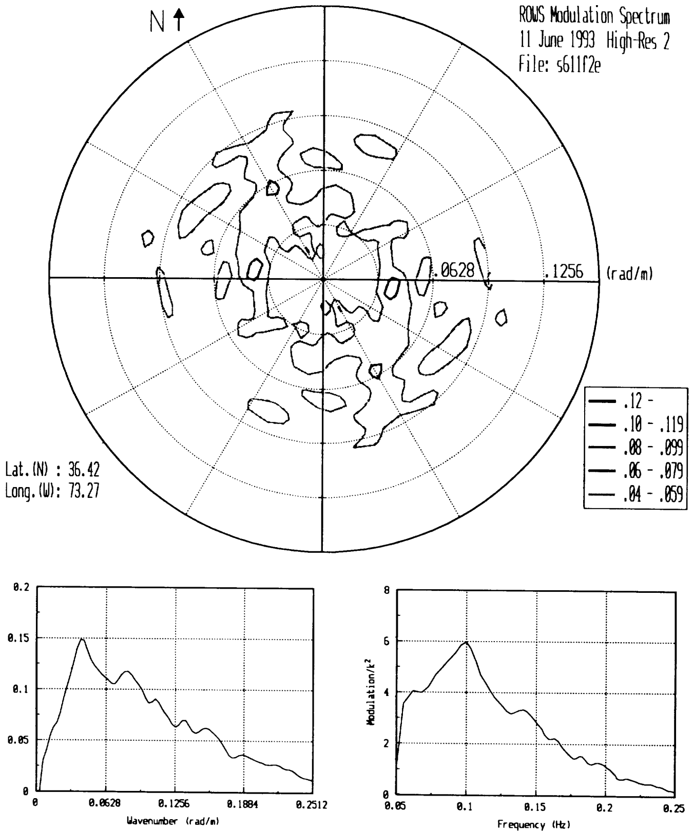
Figure 40. ROWS spectral data, file s611f2e.
