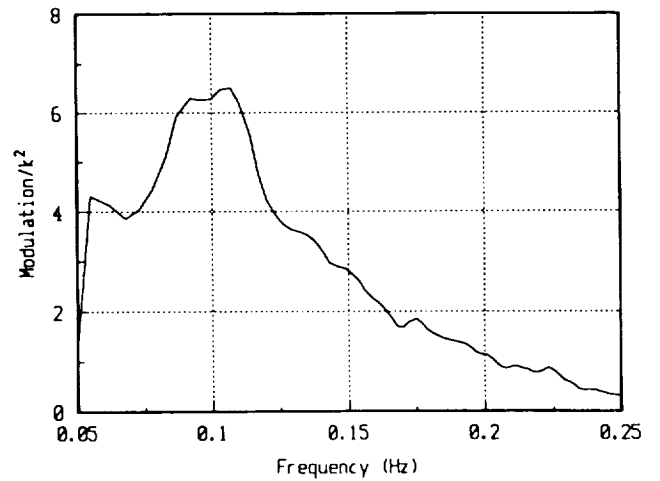
Figure 53. ROWS spectral data, file s620f2k.
