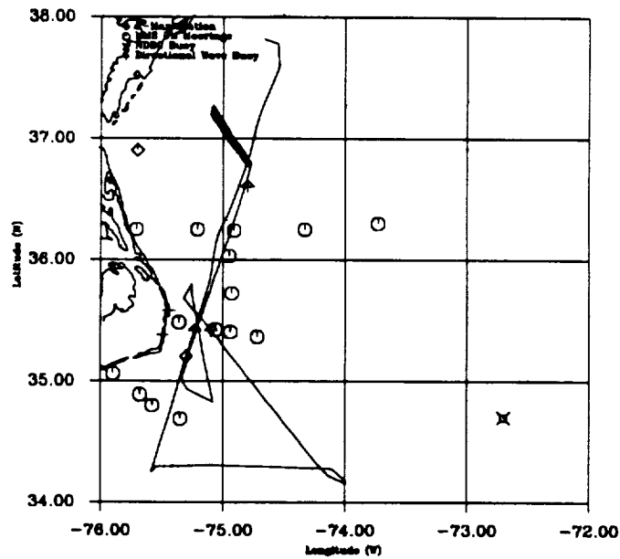
Figure 28. Altimeter mode summary, file 9, June 20, 1993.
