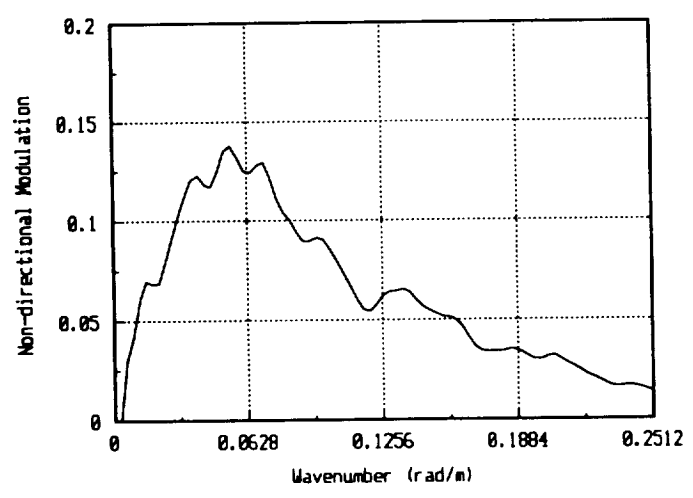
Figure 41. ROWS spectral data, file s611f2g.
