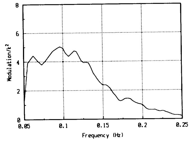
Figure 41. ROWS spectral data, file s611f2g.
