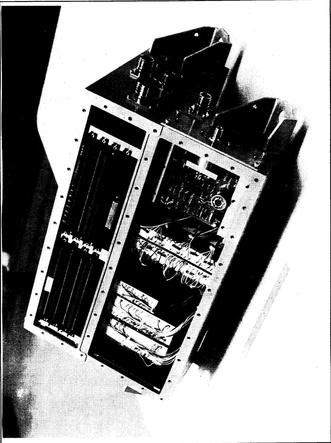
Figure 59 - EOU Assembly With Side Cover Removed
