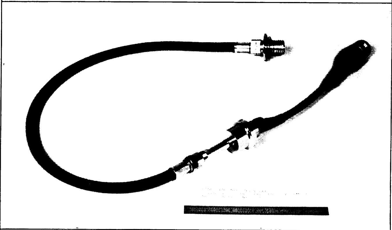
Figure 43 - Fiber Optic NL Sensor and Cable Pigtails
