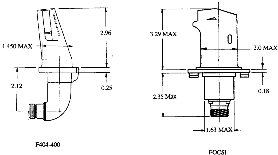
Figure 8 - T1 Temperature Sensor Housing Configurations
