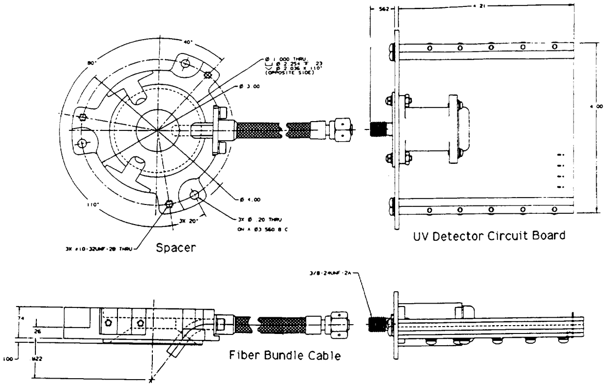
Figure 16 - A8 Flame Detector Components
