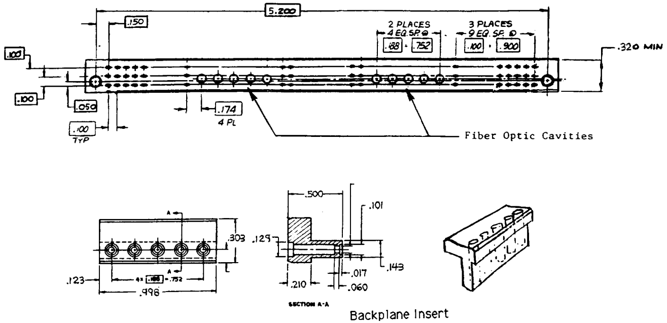
Figure 18 - Modified SEM-E Connector and Backplane Insert For Backplane Fiber Optic Terminus
