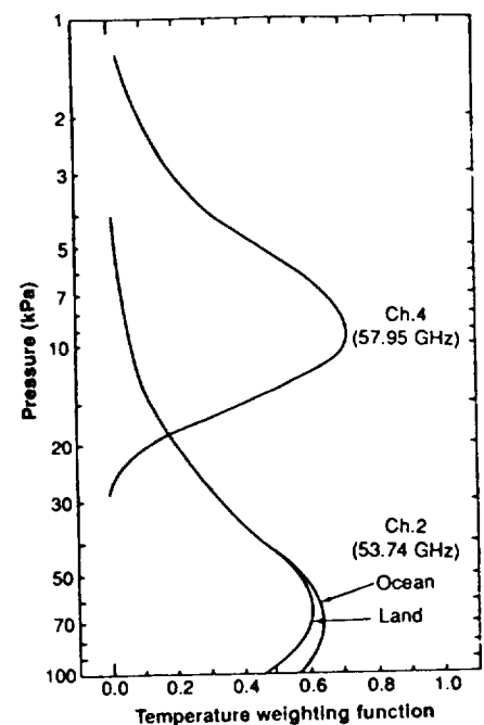
Fig. 1. Temperature weighting functions (unitless) for MSU channels 2 (mid-troposphere) and 4 (lower stratosphere). Also shown are the different channel 2 weighting functions for ocean and land surfaces, which arise because the less emissive ocean reflects more of the downwelling atmospheric radiation back upward. Sensitivity to the surface radiation itself cannot be implied from the magnitudes at the intersection of the curves with the surface. [Adapted from (6)]
