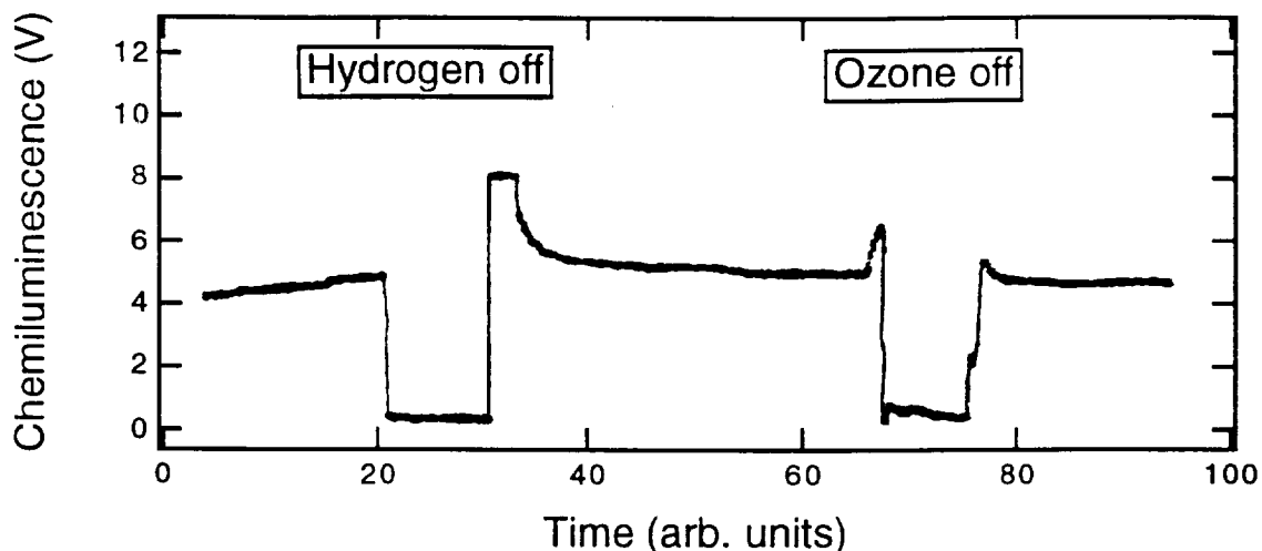
Figure 1. Trace of OH* chemiluminescence versus time. Signal disappears when either H 2 or ozone flows are turned off.
