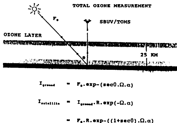
Fig. 1. Schematic diagram that shows how TOMS measures the backscattered radiation from reflecting surface. F_0 is the solar irradiance, I_{ground} is the intensity reaching to ground, I_{sat} is the measured intensity by TOMS, \Omega is total ozone, and \alpha is the ozone absorption coefficient.
