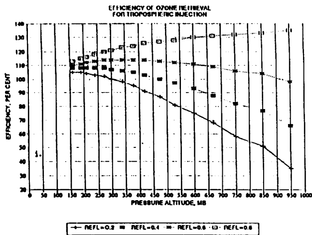
Fig. 2. The efficiency of detection for tropospheric ozone as a function of the altitude and the reflectivity of the surface (1000 mb). X-axis is the altitude in atmosphere, y-axis is the retrieval efficiency (sensitivity) of tropospheric ozone in percentage, and R is the reflectivity of the surface. The values are calculated at zero solar zenith angle, azimuthal angle, and scan angle.
