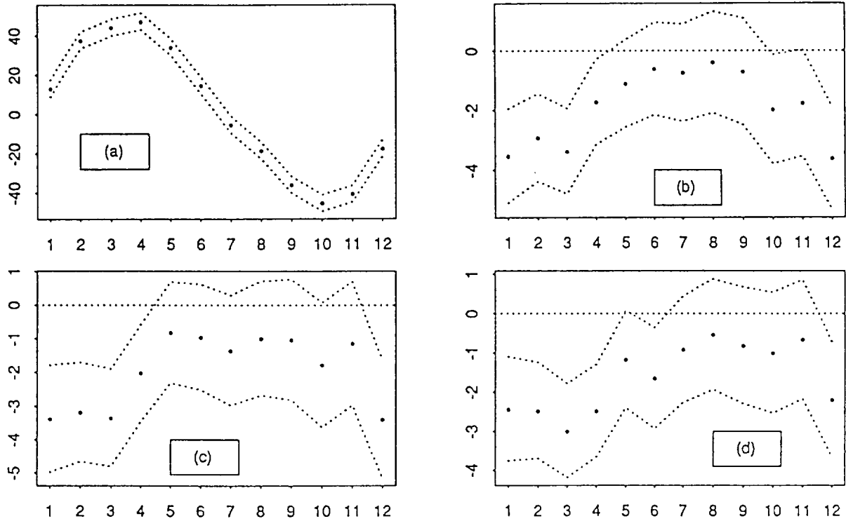
Figure 1: Total ozone series of Arosa. Labels of the abscissa: number of the calendar month. (a): Deviation of the monthly mean values (in D.U.) from the long-term annual mean value (332 D.U.). The dashed lines include the 95% confidence intervals of the monthly deviations. (b)-(d): Trends in the monthly mean values (in % per decade). The dashed lines include the 95% confidence intervals for the calculated trends which were assumed to start in Jan. 1970. (b): Model of eq. (1), ozone series 1926-91. (c): Model of eq. (1), ozone series 1947-91. (d): Model of eq. (3), ozone series 1947-91, including temperature of Mt. Säntis and the F10.7 solar flux as explanatory variables.
