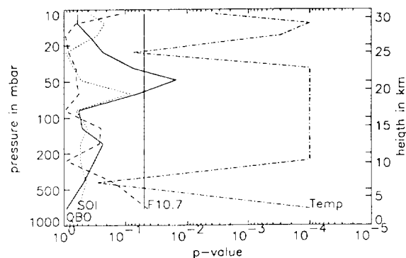
Figure 2: Significance, given as error probabilities (p-values), of the dependence of the ozone concentration on the used explanatory variables as function of the altitude. The p-value in this case is the probability that the standardized regression coefficient is smaller than the estimated value.
