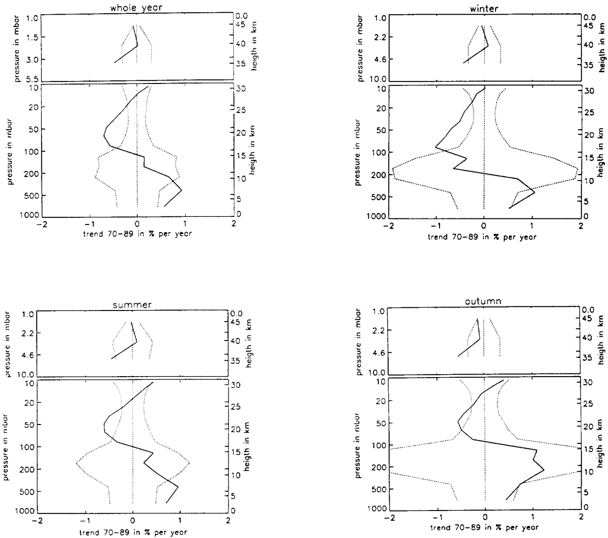
Figure 3: Trends for different altitudes deduced from the ozone balloon soundings from Payerne (1967-89) and the Umkehr-measurements from Arosa (1956-89), calculated using model of eq. (3). Trends are assumed to start on Jan., 1970. The dashed lines describe \pm 2s ( s is the standard deviation of the trends). Thus points outside the dashed line indicate trends, which are statistically significant according the t-test for regression coefficients approximately at the 5% level. a: Year around trends; b: Trends for winter (Dec. to March); c: Trends for summer (May to Aug.); d: Trends for fall (Sept. to Nov.).
