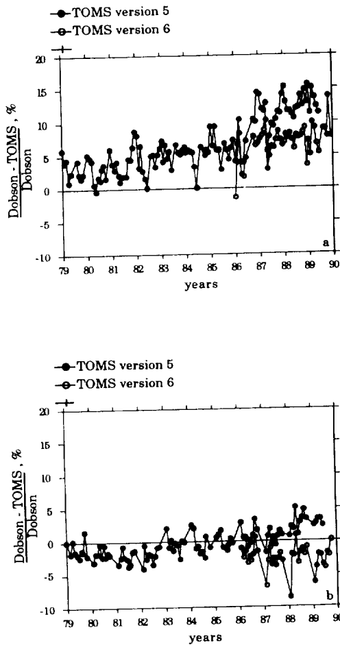
Fig. 1. Monthly mean relative differences (Dobson - TOMS) / Dobson at the ground stations in (a) Oslo and (b) Reykjavik. TOMS version 5 (solid circles) and version 6 (open circles), markers indicate new year.
