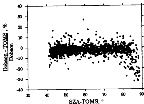
Fig. 5. Relative differences in total ozone at Reykjavik versus the solar zenith angle (SZA) at the time of TOMS measurements.
