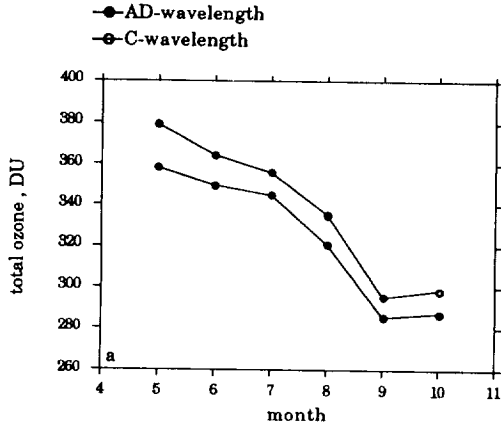
Fig. 2. Monthly mean total ozone from Dobson measurements at Oslo with the AD wavelength double pair (solid circles) and C wavelength pair (open circles) in 1990.
