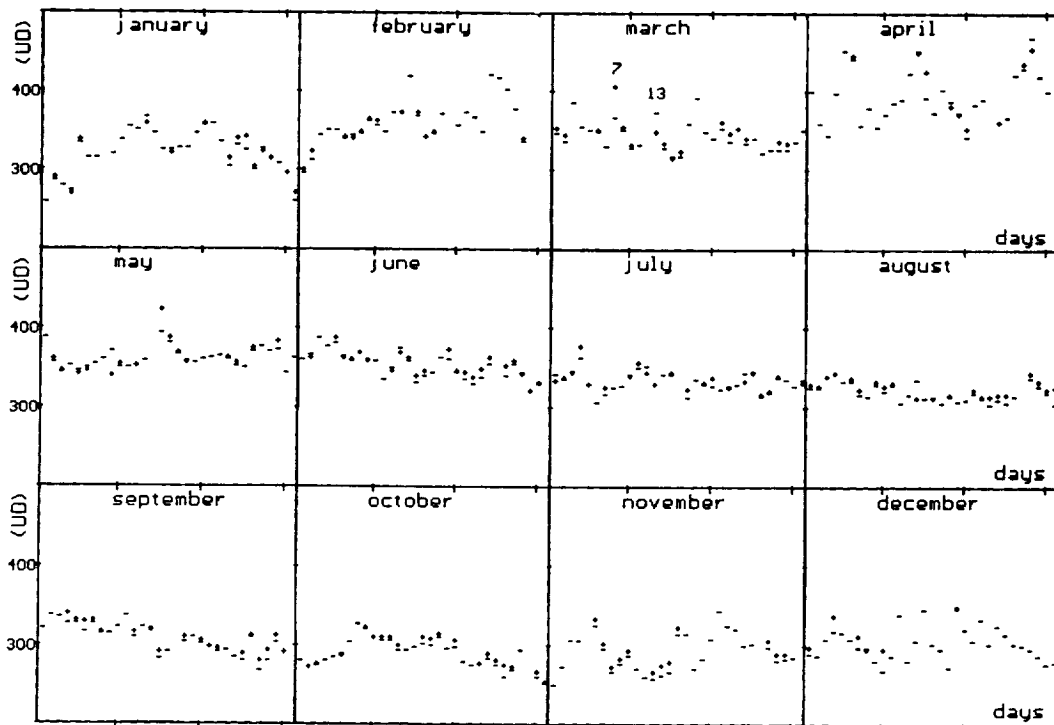
Fig 3 : Daily Total Ozone: comparison between TOMS (-) and DOBSON-OHP (+) measurements in 1989
