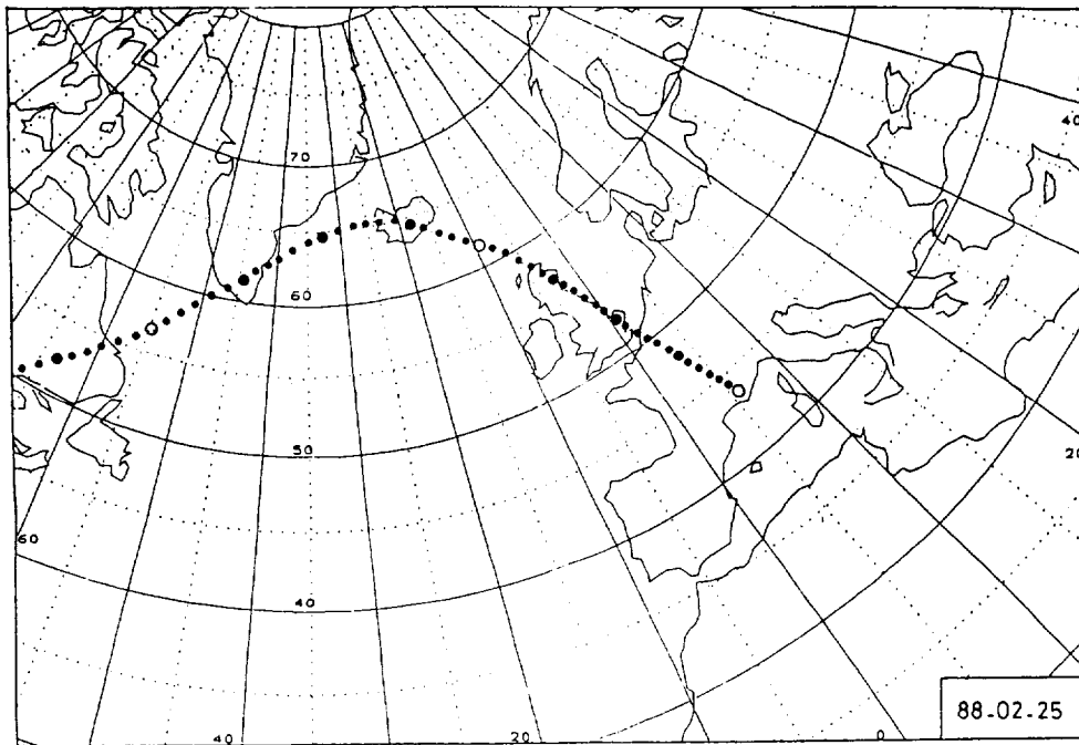
Fig 5 : Air mass backward trajectory ending at O.H.P. 1988-02-25-12UT. Ending pressure level 70hPa. o-o: 24h ●-●: 6h - - -: 1h
