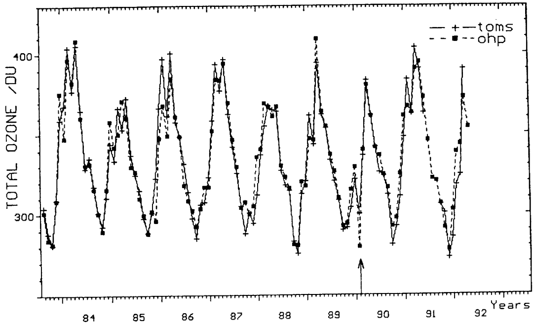
Fig 1 : Monthly mean Total Ozone : comparison between TOMS and DOBSON -OHP (September 1983 - April 1992)
