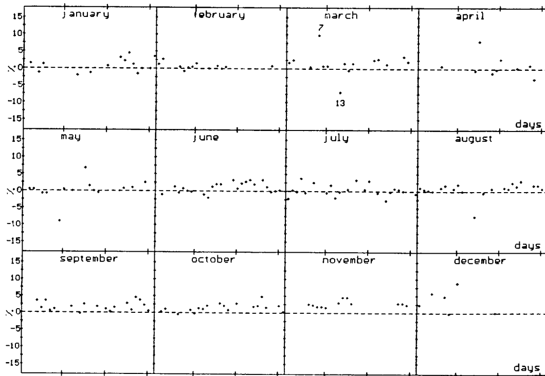
Fig 4 : Daily Total Ozone: Relative differences between TOMS and OHP in 1989. (OHP - TOMS) / OHP (%)
