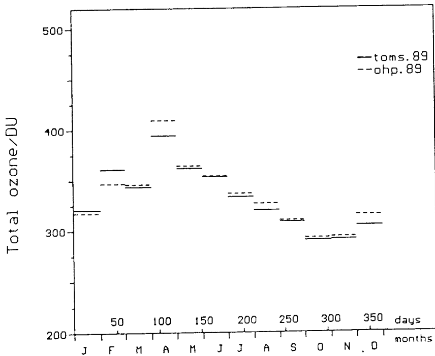
Fig 2 : Monthly mean Total Ozone: comparison between TOMS and DOBSON-OHP measurements in 1989
