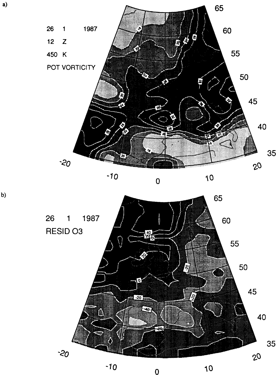
Fig.5 a)Potential vorticity field at 450 K potential temperature, 12h 26 Jan 1987 in units of \mu\text{Km}^2(\text{kgs})^{-1} , derived from ECMWF operational analyses. Note the tongue of high PV extending southwestwards between 40^\circ and 50^\circ\text{N} . b)Residual ozone field in DU for the same time. This was calculated by subtracting from the actual total ozone at each point (measured by TOMS) the value predicted from the regression equation between total ozone and absolute vorticity derived on the 17th January. Note negative residuals corresponding to the PV tongue in a): the polar vortex shows up as a region of lower total ozone once tropopause-level disturbances are removed.
