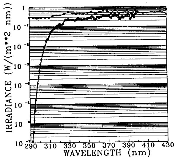
Fig. 3 Solar global radiation at Potsdam (52° 22' N, 13° 5' E) on October 11, 1991, 11.24 CET, \theta = 59.631^\circ □—□ extraterrestrial radiation from CIMO (1981) corrected for solar zenith angle and distance sun-earth ▲—▲ measurements of global solar radiation taken with the spectrometer OL 752/10 at Potsdam 18 m above the ground, clear sky ○—○ model calculation of global radiation (direct + diffuse) with O_3 = 271 D and an aerosol optical thickness of \tau = 0.4 with \lambda = 350 nm
