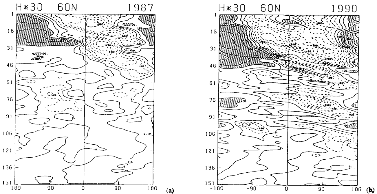
Fig.4 : Longitude-time diagram for the asymmetric part of 30 mb heights at 60N for (a) 1987 and (b) 1990.
