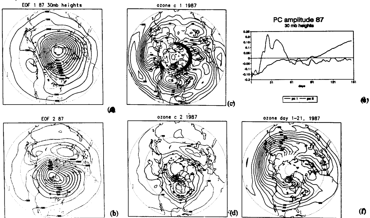
Fig.2: (a) EOF 1 and (b) EOF 2 for 30 mb heights for 1987. (c) C_1 , (d) C_2 , (e) Principal components PC 1 and 2 associated with EOF 1 and 2, and (f) total ozone averaged from January 1 to 21, 87
