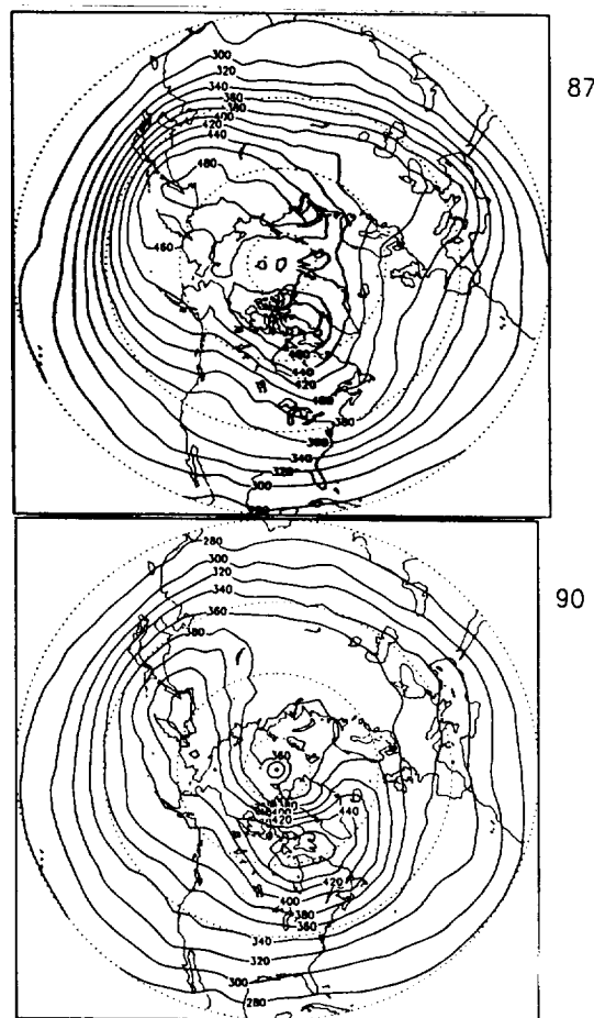
Fig.1: Total column ozone averaged from February to April for (a) 1987 and (b) 1990. Contour interval 20DU
