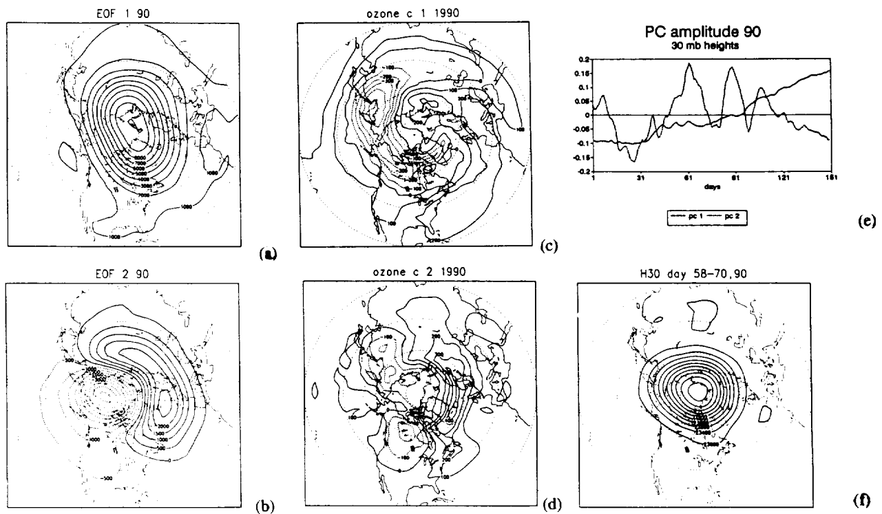
Fig.3: (a) - (e) Same as Fig.2, but for 1990, (f) 30 mb heights averaged over February 27 -March 11, 90
