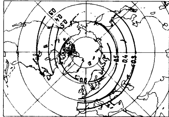
Fig.4. The partial correlation coefficient (relative to ozone - 300 mb geopotential correlation) of total ozone and 10 mb geopotential for Winter.
