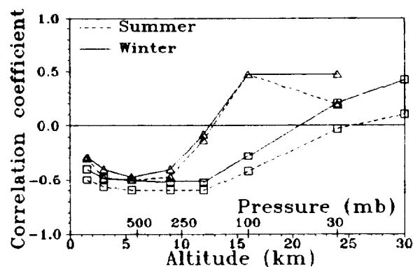
Fig. 1. Correlation coefficients between total ozone and temperature (▲) and between total ozone and geopotential high (◻) for Central Europe.
