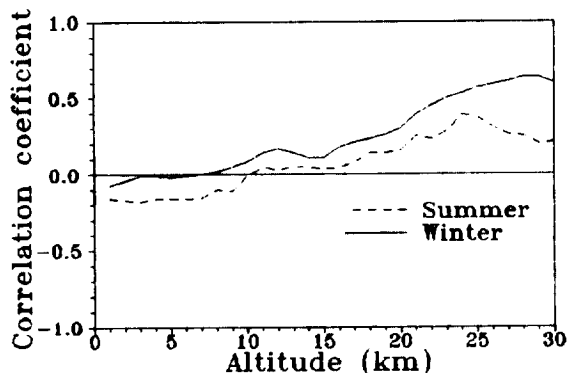
Fig. 6. Correlation coefficient between the temperature at the 24 km level (30mb) and ozone concentration at different altitudes for Hohenpeissenberg.
