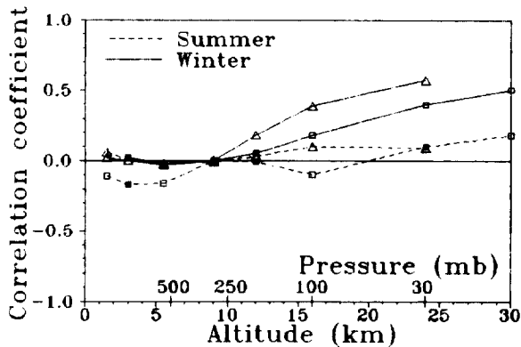
Fig. 3. Partial correlation coefficients (relative to ozone - 300 mb geopotential correlation) between total ozone and temperature ( \Delta ) and between total ozone and geopotential ( \square ) for Central Europe.
