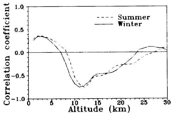
Fig. 5. Correlation coefficient between the temperature at the 6 km level (500mb) and ozone concentration at different altitudes for Hohenpeissenberg.
