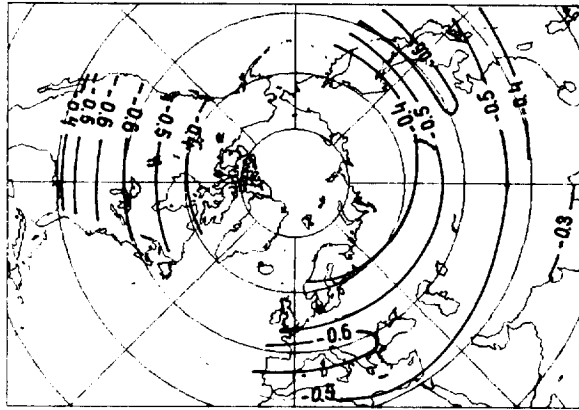
Fig. 2. Correlation coefficient of total ozone and 300 mb geopotential high for Winter.
