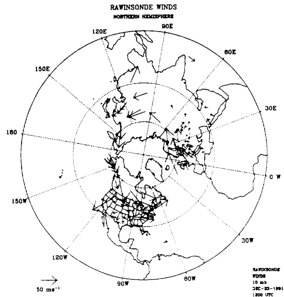
Figure 2. 10-mb observed 1200 UTC rawinsonde winds for December 23, 1991. Units: \text{ms}^{-1} .
