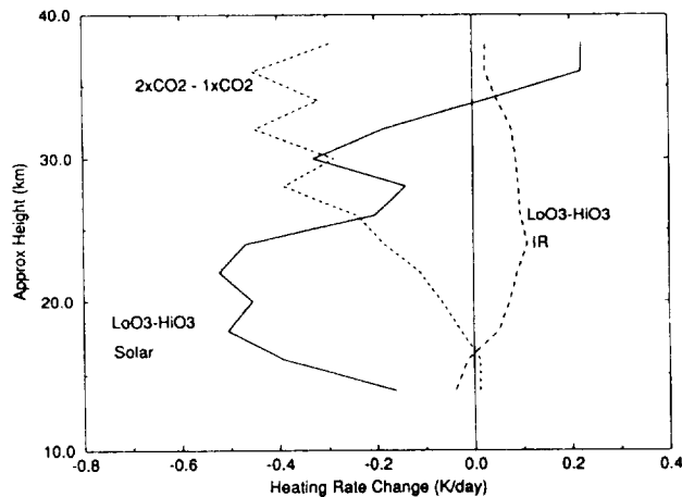
Fig. 4. Effect of changes in ozone and carbon dioxide on heating rates. A temperature profile from the present day CO 2 simulation on 4 April is chosen, and the effect of doubling CO 2 and depleting ozone (separated into solar and thermal infrared effects) are shown. The depleted ozone profile corresponds to the grid point of minimum ozone on 4 April of the double CO 2 simulation.
