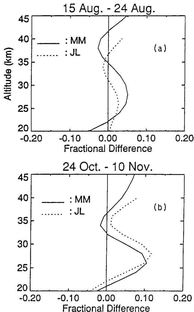
Figure 3. Interannual ozone changes: the fractional difference in ozone between two periods in 1990 and corresponding periods in 1989 as measured by the JPL lidar and by the microwave instrument. The lidar data have been smoothed to the resolution of the microwave measurement using the microwave averaging kernels.
