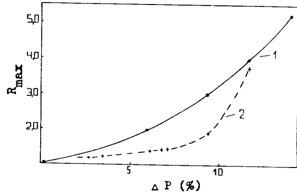
Fig 6. Minimum's depth \Delta P vs maximum value of the lidar profile R_{max} after theoretical (1) and experimental (2) data.
