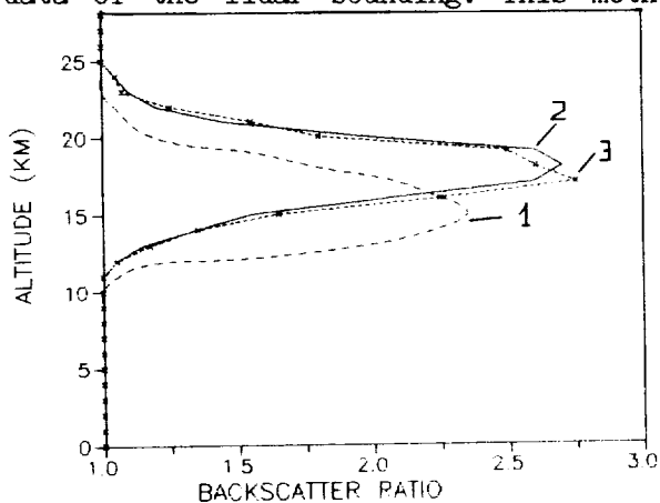
Fig. 8. Solution of the direct and inverse problem for the closed scheme: 1- average backscatter coefficient's profile, 2- set profile for the direct problem, 3- result of the retrieval.
