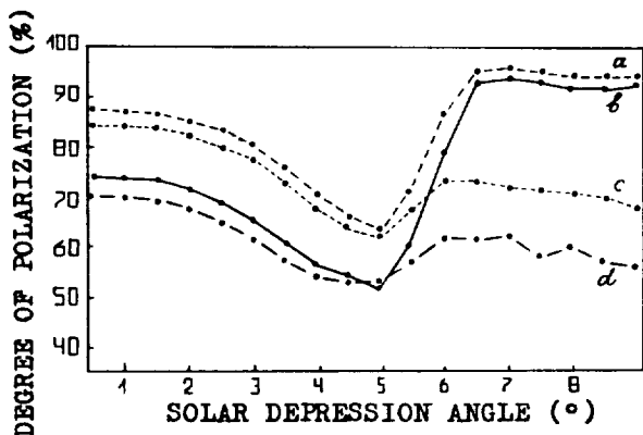
Fig. 7. Calculations of the degree of polarization for two models ( R = \frac{4.5}{r_{max}} ): with the modal radius of the aerosol particles 0,075 (a,c) and 0,15 (b,d) in cases when the single scattering approximation was applied (a,b) and when the multiple scattering was taken into account (c,d).
