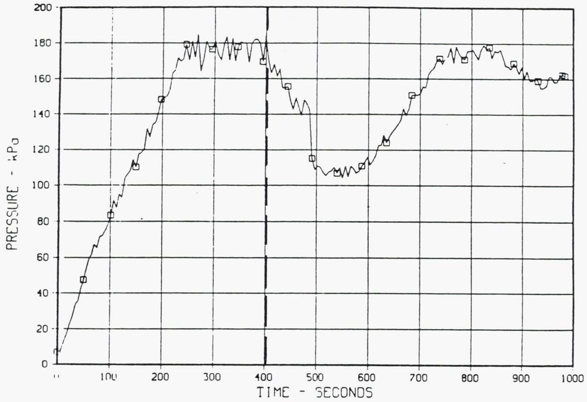
Figure 4-5. Pressure Profile for Test 2.0-6; \text{GH}_2 Pressurization of TPLH 2
