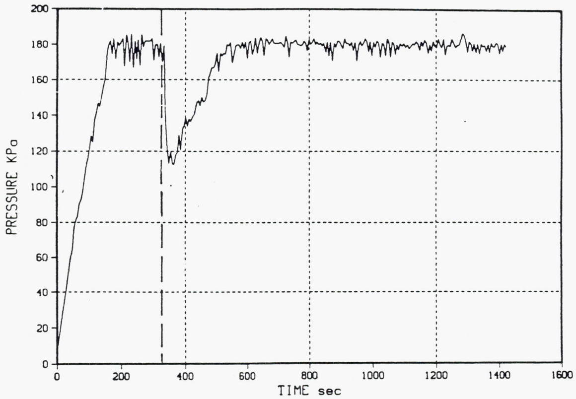
Figure 4-6. Pressure Profile for Test 2.0-17; \text{GH}_2 Pressurization of SH 2
