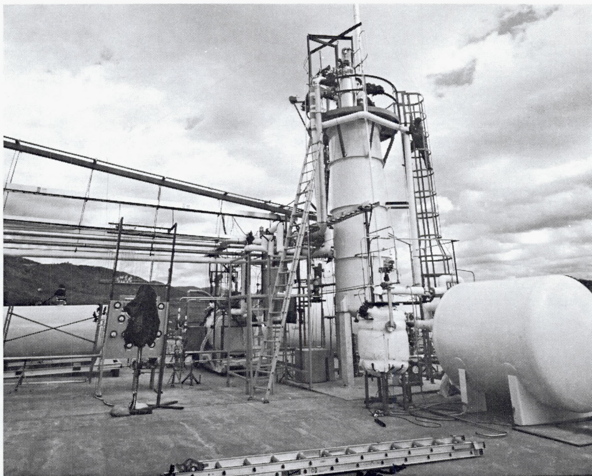
Figure 3-15. Pressurant Heat Exchangers and Slush Generator View
