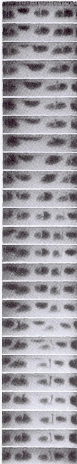
FIG. 99. Time sequence of twenty-five smoke visualization photographs illustrating the emergence of vortex pairs from near-wall regions for De=100 at a streamwise location 95^{\circ} from the start of curvature. All other figure details are the same as for Fig. 92 except that the time interval between photographs is 1/10 second.
