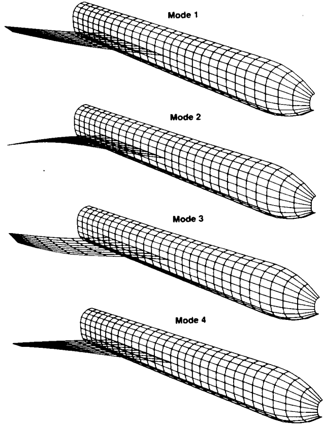
Fig. 11 First four natural modes of the wing-body configuration.
