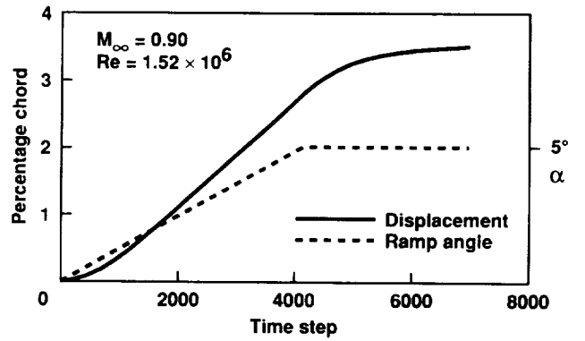
Fig. 14 Static aeroelastic displacements of wing-tip leading edge
