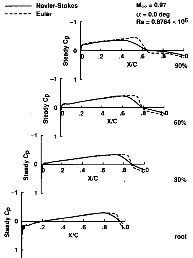
Fig. 6 Comparison of transonic steady pressures from Euler and Navier-stokes solutions.
