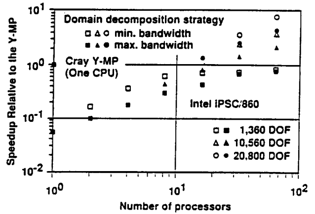
Fig. 11: Computational performance of the structural domain in ENSAERO with various problem sizes and domain decompositions on the Intel iPSC/860
