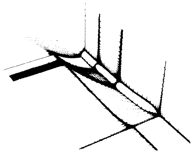
Fig. 12 Deformed surface and field grids.
