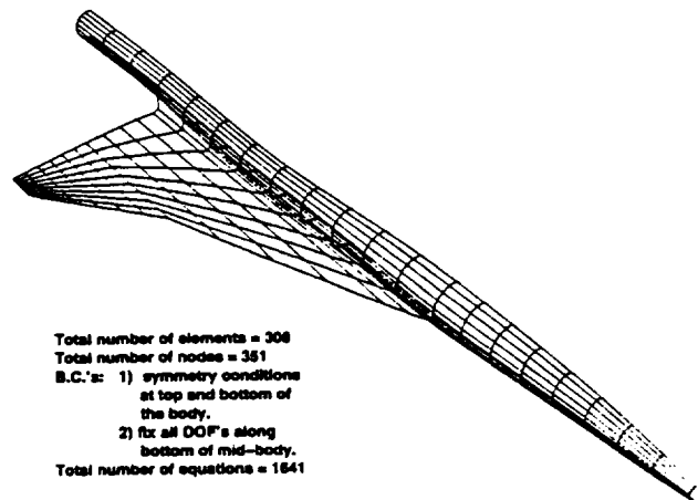
Fig. 8: Finite-element modeling of the wing-body configuration.
