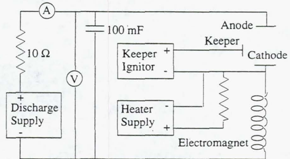
Fig. 4 SPT Electrical Schematic
