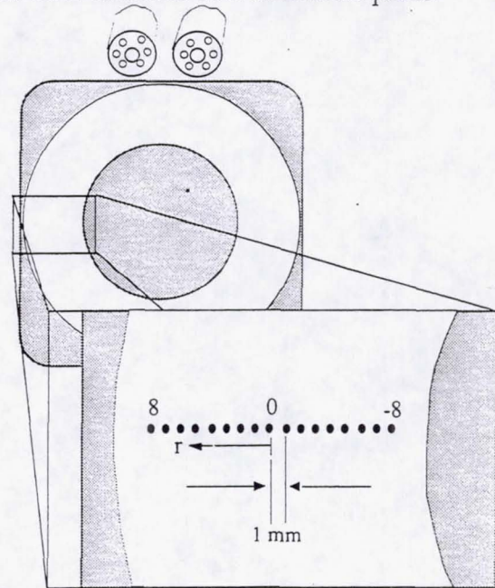
Fig. 6 Measurement Locations for Axial and Radial Velocity Determination
