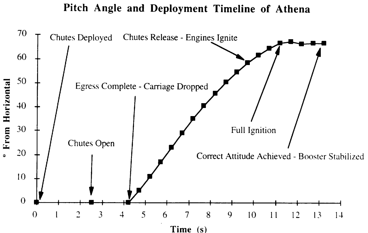
Figure 8.5: Pitch angle during extraction
