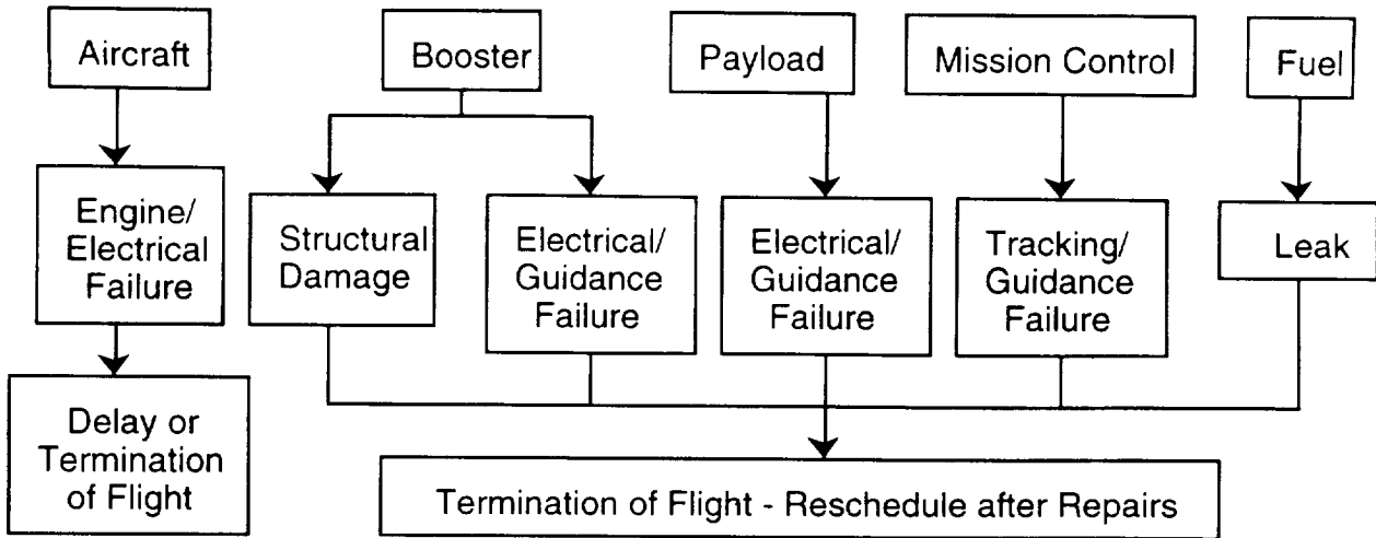
Figure 3.5: Abort Scenarios Prior to Launch
