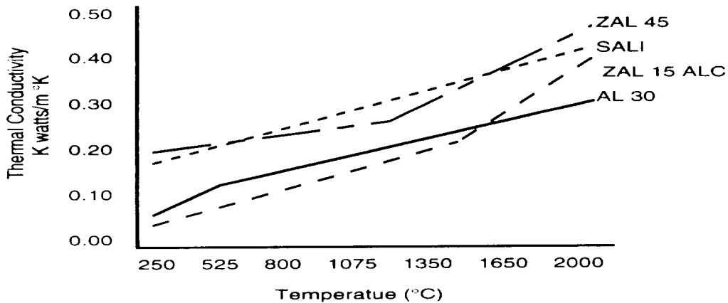
Figure 7.5: Comparison of Thermal Conductivity for Various Fibrous Ceramics Over a Varying Temperature
