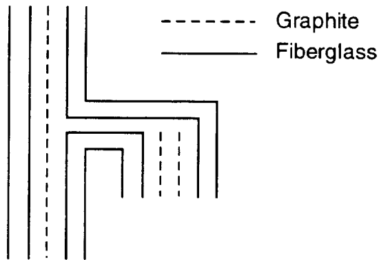
Conf. 3: Integrally Stiffened Laminate Structure
