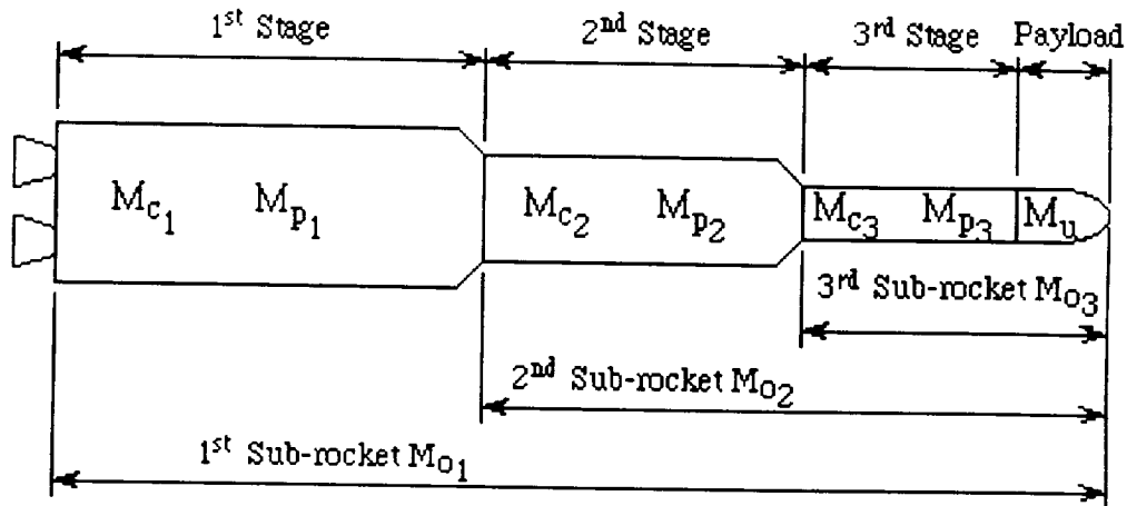
Figure 4.2: Nomenclature for a Three-Stage Rocket
