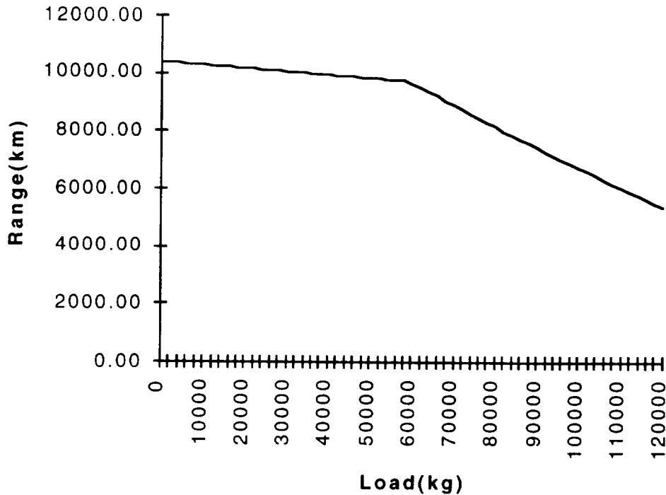
Figure 2.7: Graph of Chimaera Range vs. Payload (raw data for Figure 2.7 can be found in the Appendix A.2)
