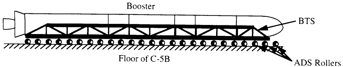
Figure 7.12: Schematic of BTS
