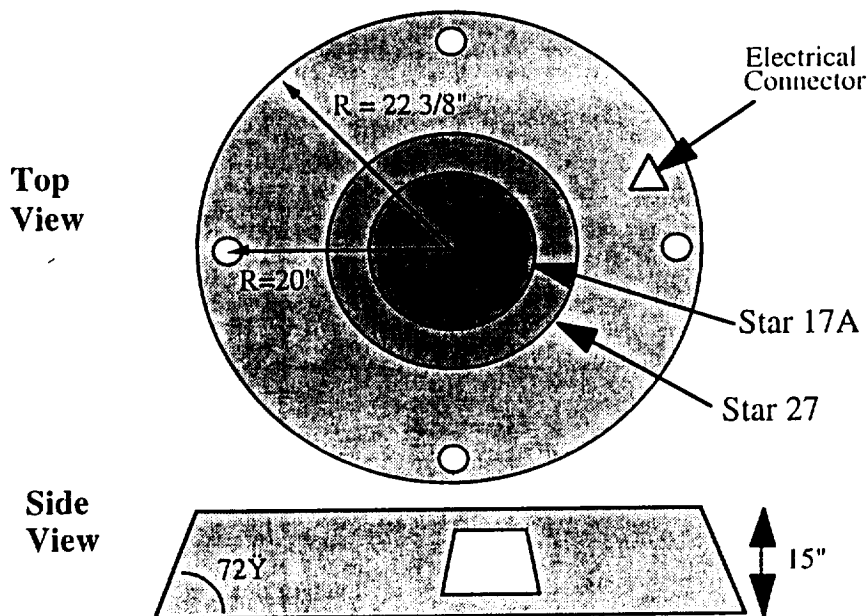
Figure 1. Payload Support Bulkhead
