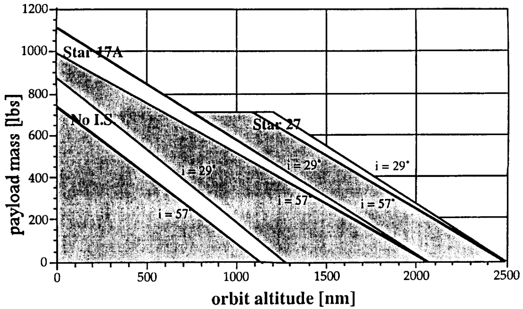
Figure B.1.2. Launch Performance at Cape Canaveral Launch Site
