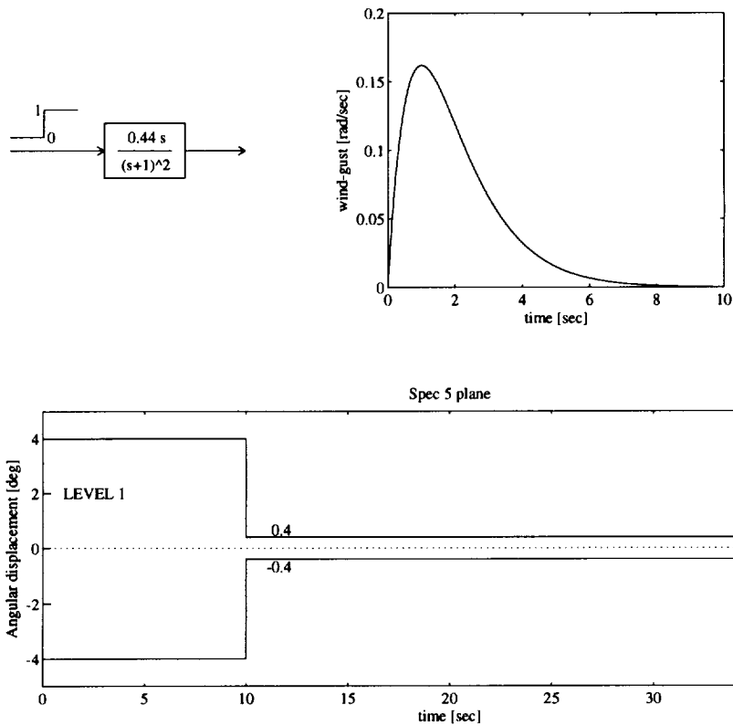
Figure 4.8: Spec 5: Wind-gust rejection - required envelope
