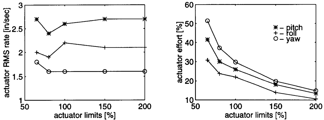
Figure 6.11: Actuator effort as a function of \mu .
