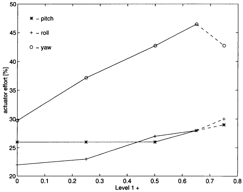
Figure 6.6: Actuator effort as a function of #.
