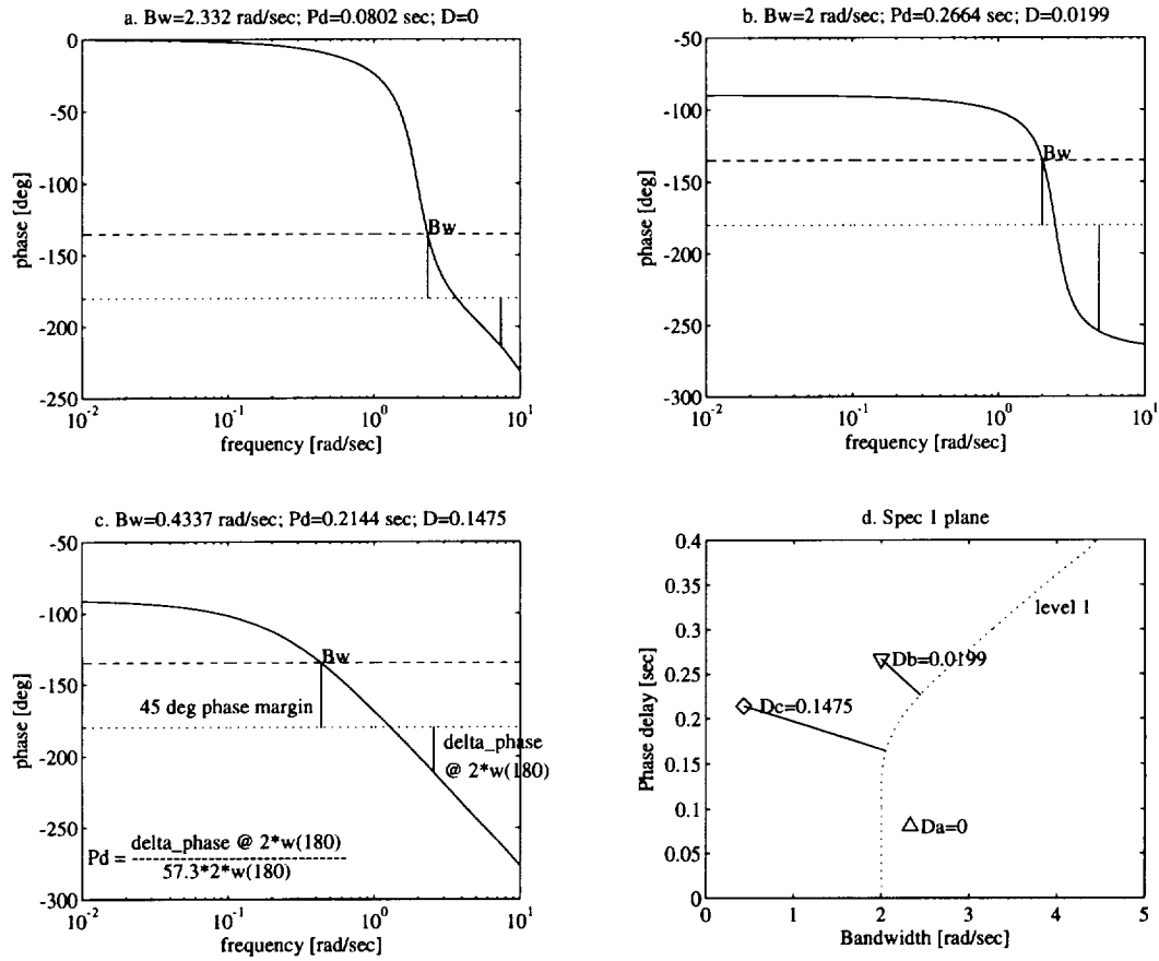
Figure 4.2: Spec 1: Bandwidth vs. Phase-delay (a-c) Bode phase plot, bandwidth and phase-delay of three examples. (d) their D measures in the Spec 1 plane.
