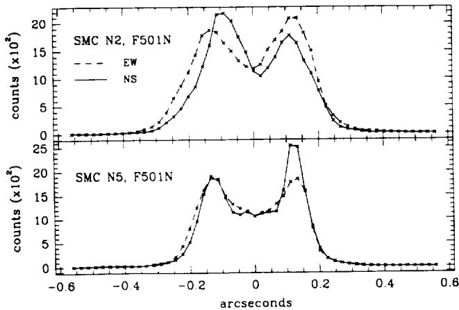
FIG. 2.—Intensity cross-sections through the center of the deconvolved F501N image of SMC N2 (top) and N5 (bottom) in the east-west and north-south directions. Each cross section is an average of 3 adjacent pixels normal to the scan direction. The intensity scale is in units of FOC counts in the deconvolved image.
