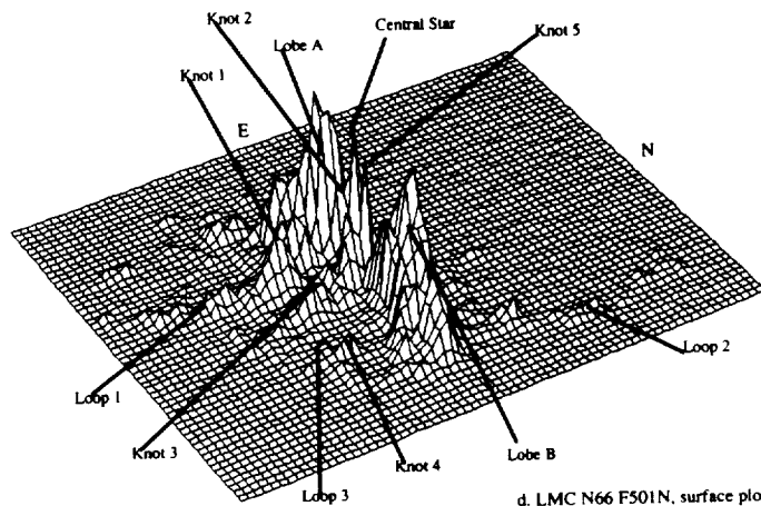
d. LMC N66 F501N, surface plot
