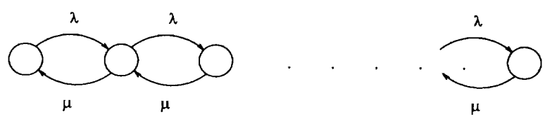
Figure 4: Birth-Death Markov Chain
