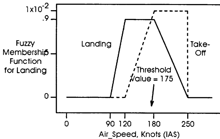
Figure 3. Membership Functions for Takeoff/Landing.
