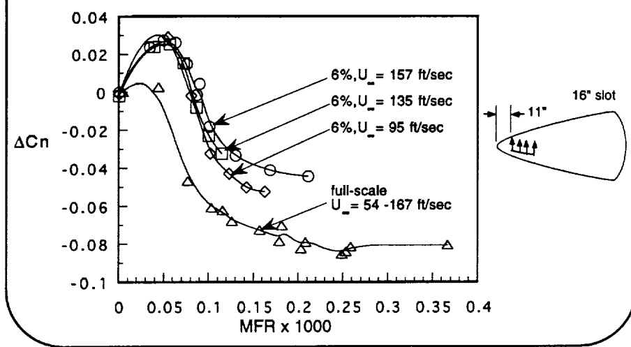
6% Scale and Full-Scale Results, \alpha = 50^\circ , \beta = 0^\circ
