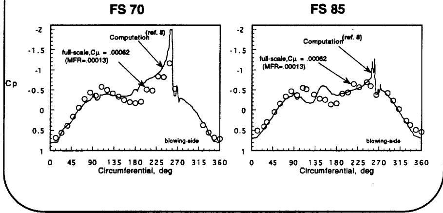
Pressure Distributions at \alpha = 30^\circ, \beta = 0^\circ
