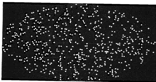
Gamma ray bursts detected by the Compton Gamma Ray Observatory
