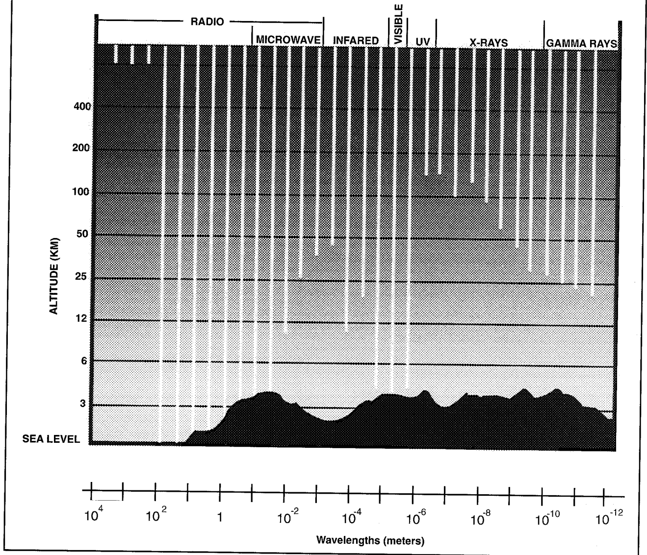
Figure 2. Transparency of Earth's Atmosphere
