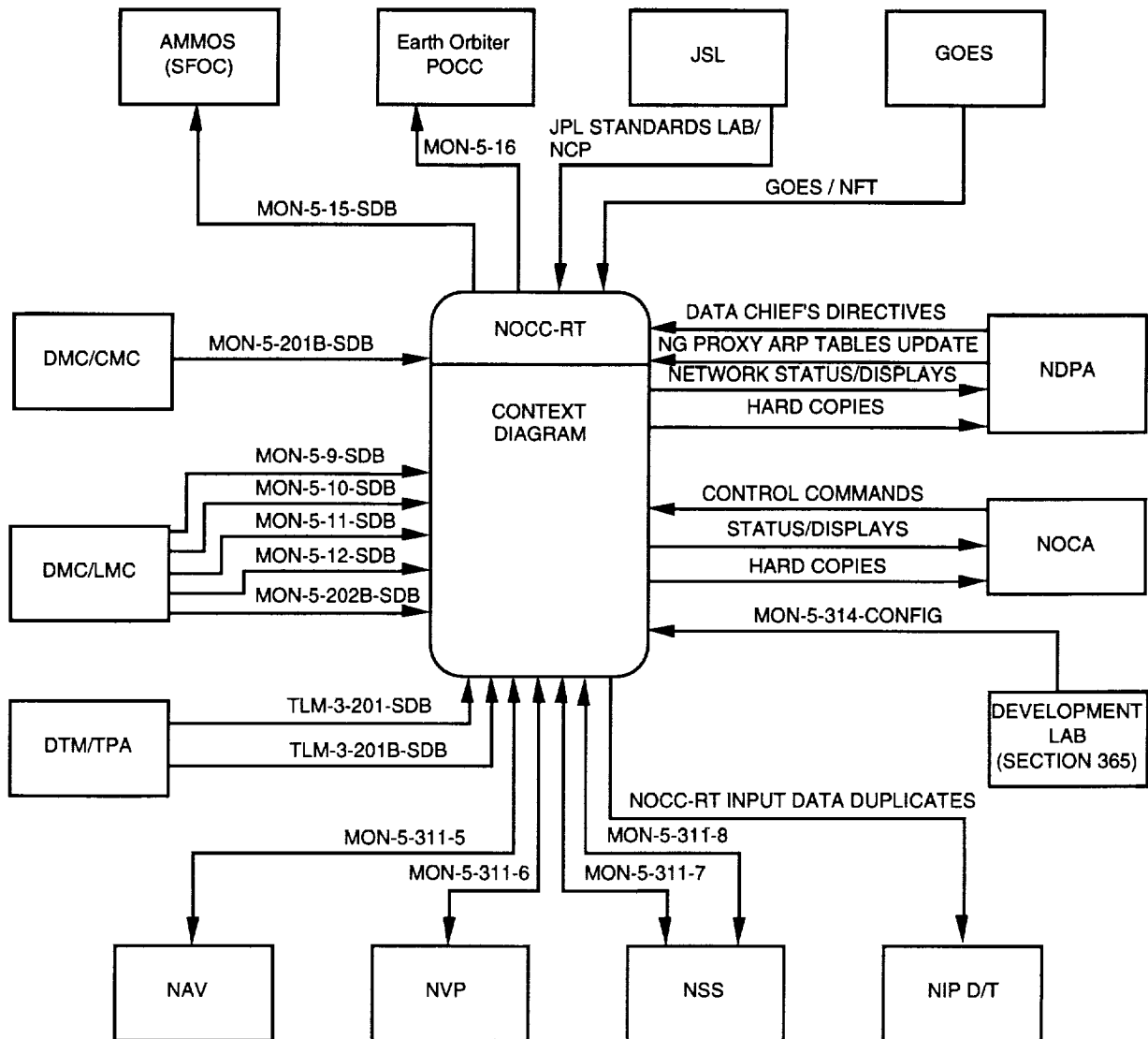
Fig. 1. NOCC-RT context diagram (Phase I).
