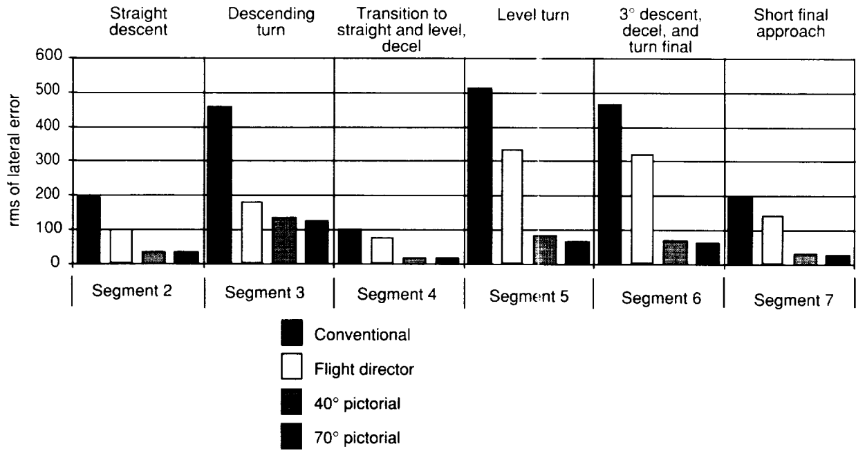
Figure 22. Mean lateral errors (for all pilots) per display concept and condition for each path segment.
