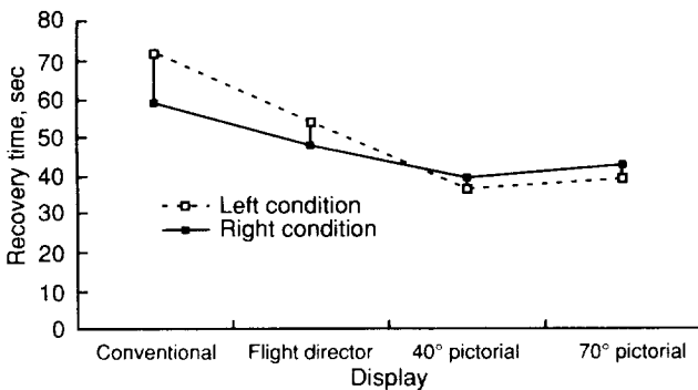
Figure 17. Offset Scenario second-order interaction between displays and scenario conditions; mean times to recover to intended flight path per display concept and condition.
