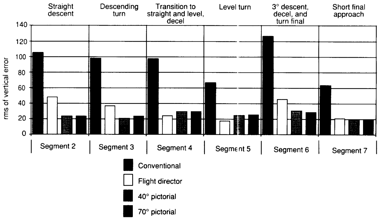
Figure 23. Mean vertical errors (for all pilots) per display concept and condition for each path segment.
