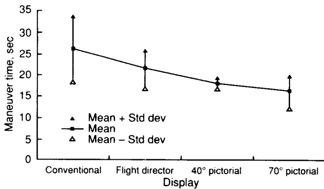
Figure 15. Runway Blunder Scenario mean times to maneuver since detection.
