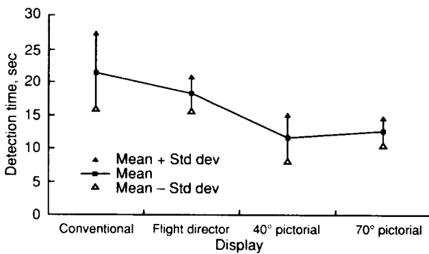
Figure 14. Runway Blunder Scenario mean detection times per display concept and condition.
