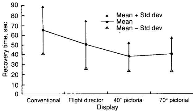
Figure 16. Offset Scenario mean times to recover to intended flight path per display concept and condition.
