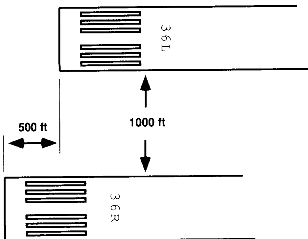
Figure 8. Offset, parallel runways.
