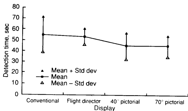
Figure 11. Traffic Conflict Scenario mean detection times per display concept and condition.
