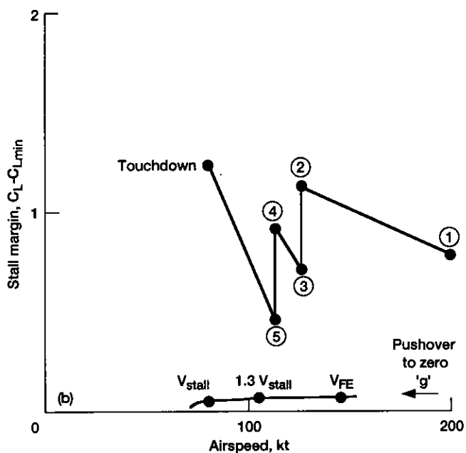
Figure 18.—Stall margins for the flight conditions shown on figure 16 and for the pushover to zero 'g' maneuver (ref. 22). (a) Wing. (b) Tail.
