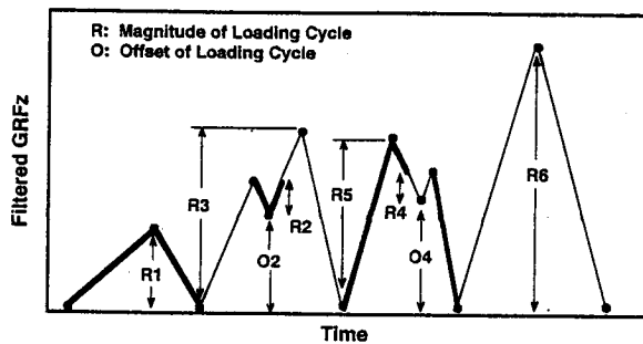
Figure 3. Illustration of the post-processing "rainflow" cycle counting algorithm.
