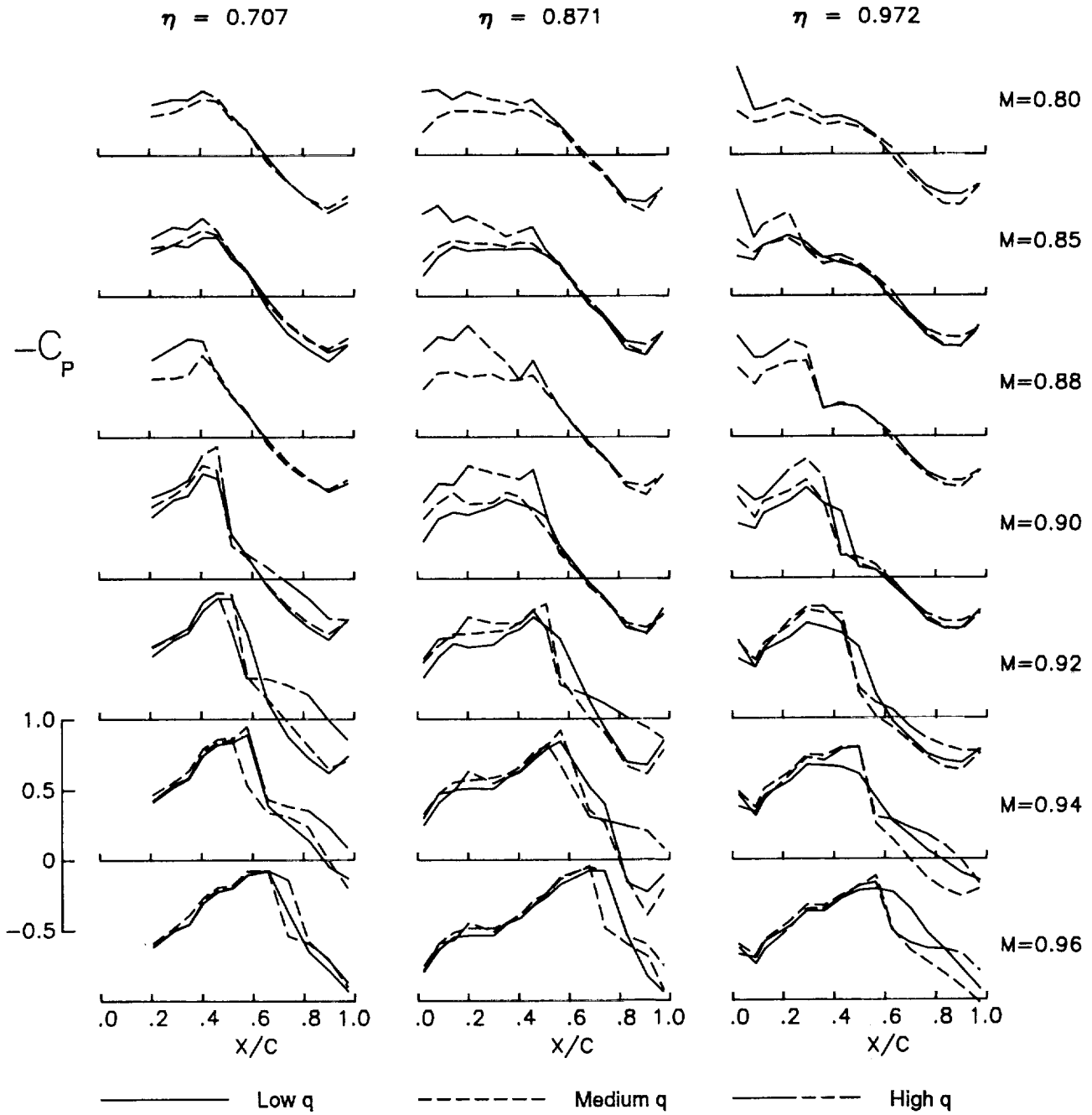
(b) Lower-surface data.
