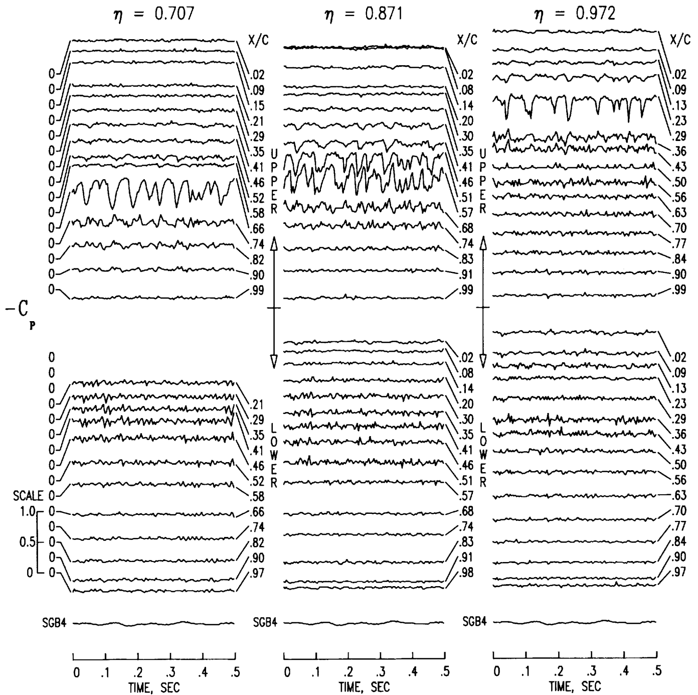
(b) Tab point 92. M = 0.85 ; q = 135.3 psf.
