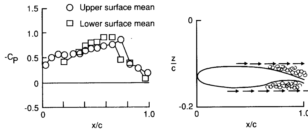
(c) Detached flow on upper and lower surface. M = 0.96 ; \eta = 0.707 ; q = 161.7 psf. (See fig. 18(g).)
