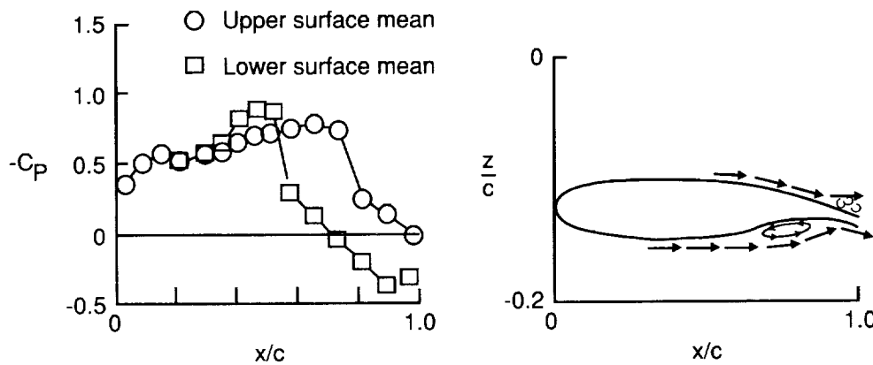
(b) Upper-surface trailing-edge flow separation and separation bubble on lower surface. M = 0.92 ; \eta = 0.707 ; q = 152.5 psf. (See fig. 18(e).)
