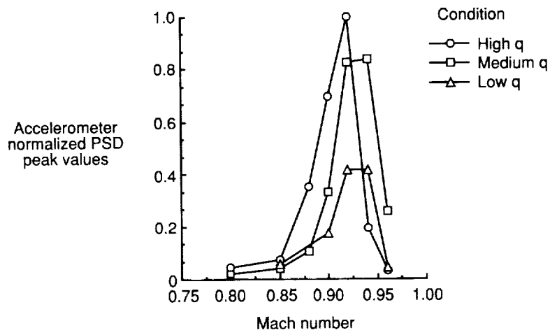
Figure 7. Maximum PSD peak responses from accelerometer 9.
