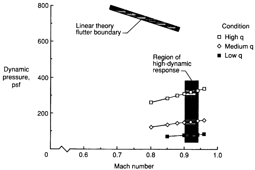
Figure 4. Test conditions.
