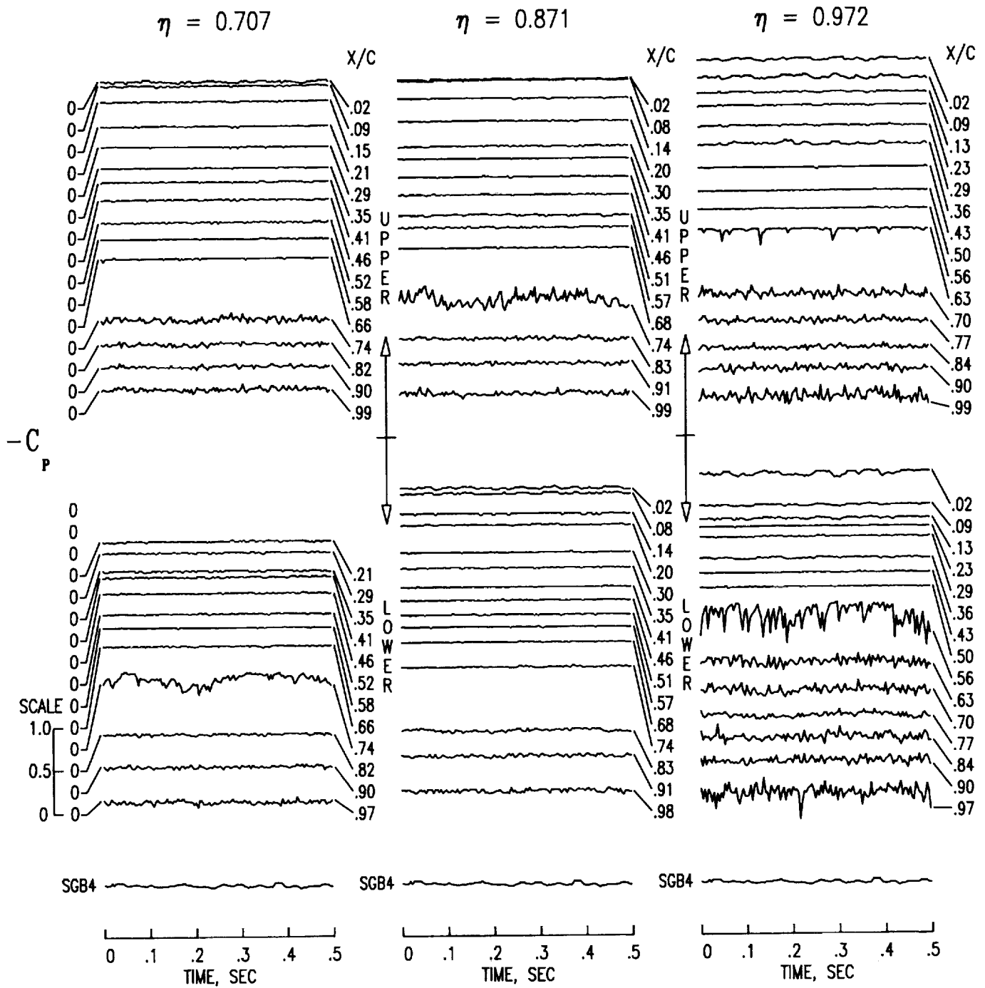
(g) Tab point 205. M = 0.96 ; q = 336.7 psf.
