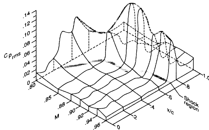
Figure 25. Pressure coefficient rms values for section of 3-D ARW-2 flexible supercritical wing. Leading-edge sweep = 28.8^\circ ; Re = 2.6 \times 10^6 ; \alpha = 2^\circ ; \eta = 0.871 .
