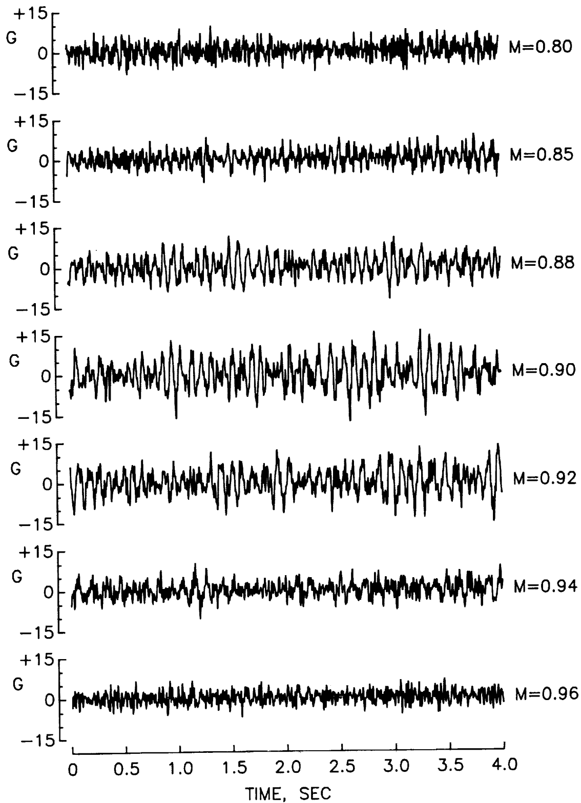
(c) Data from accelerometer 9 for high q conditions. \alpha = 0^\circ .
