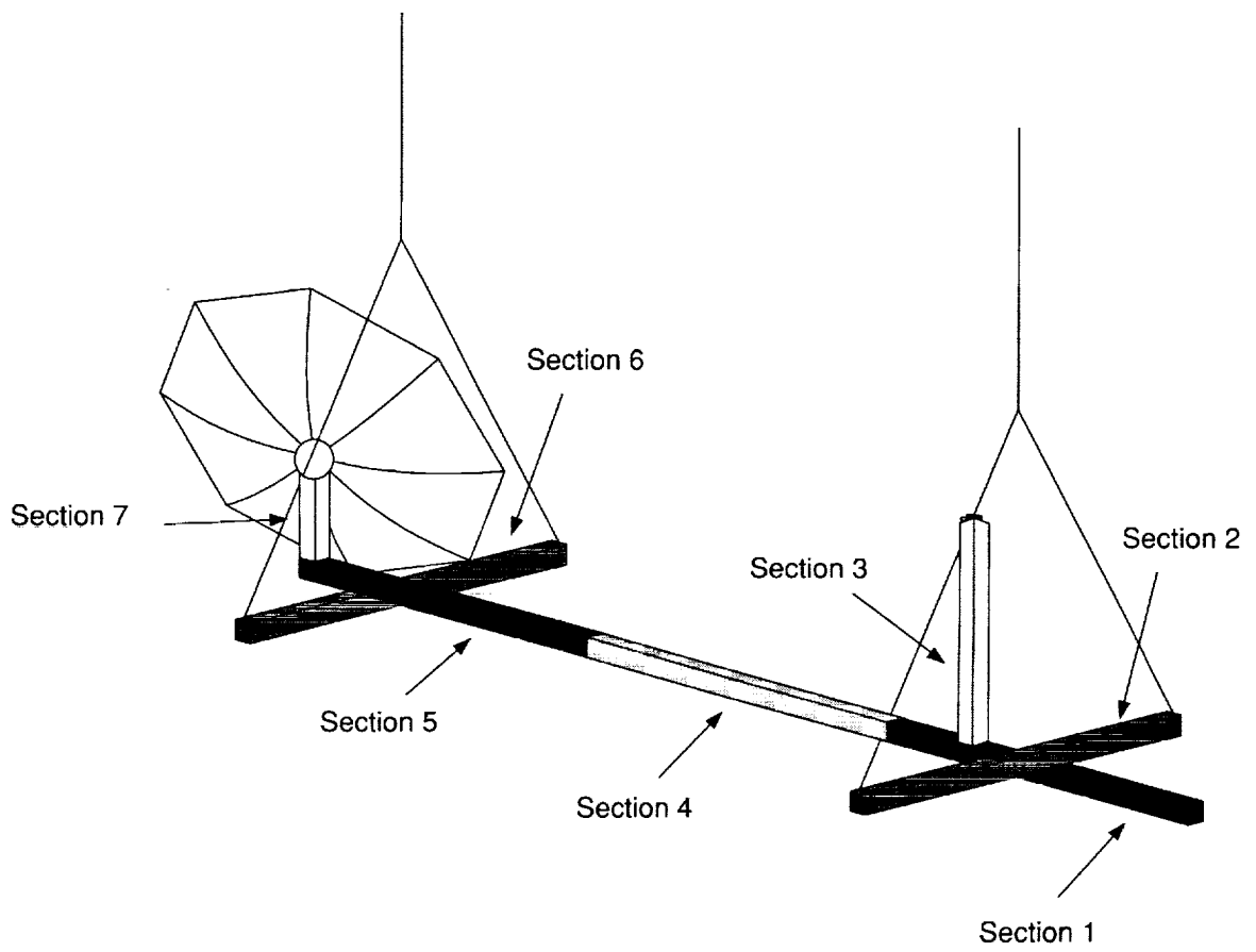
Figure 6. Seven sections of CEM model for integrated redesign.
