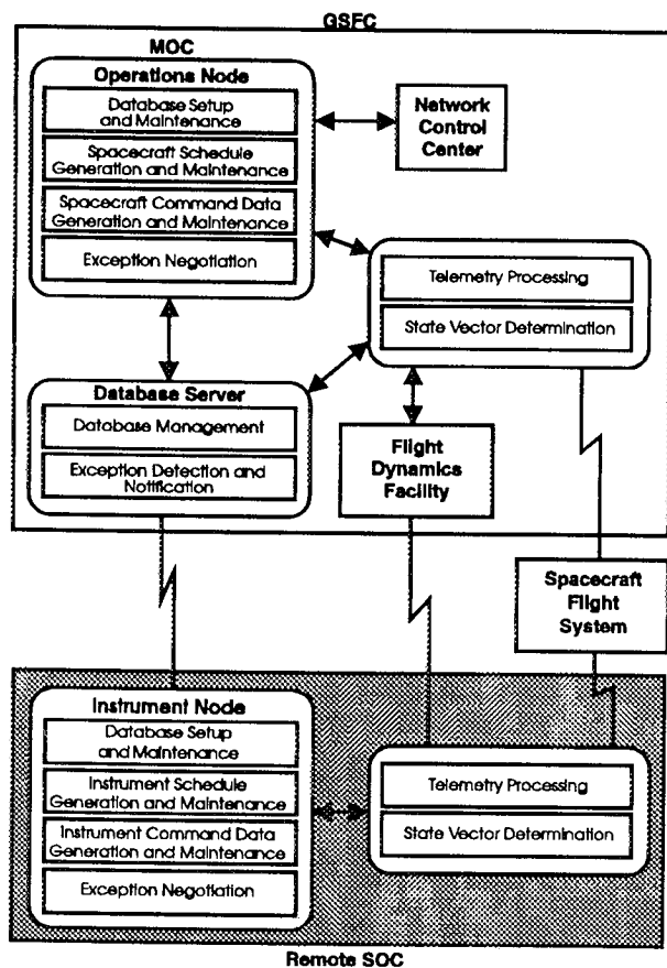
Figure 2. Architecture
