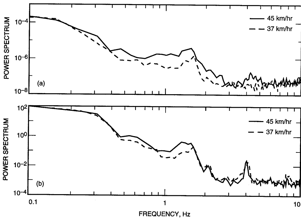
Fig. 9. Power spectra for yaw angle 90 deg and elevation angle 10 deg: (a) azimuth encoder and (b) azimuth torque.
