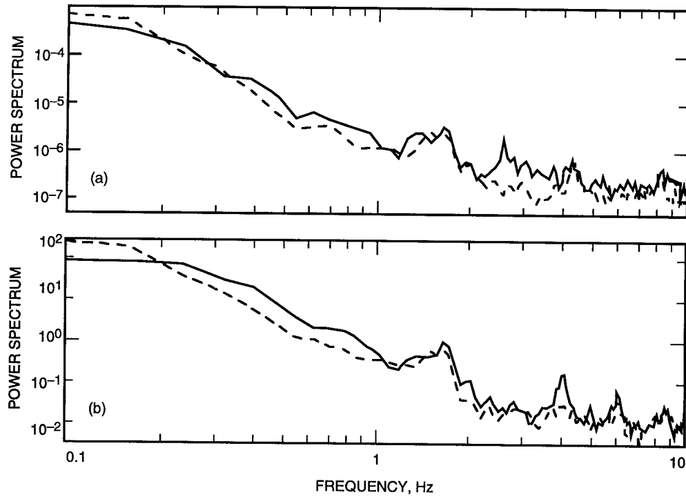
Fig. 11. Power spectra for yaw angle 180 deg and elevation angle 78 deg (solid line) and 20 deg (dashed line): (a) elevation encoder and (b) elevation torque.
