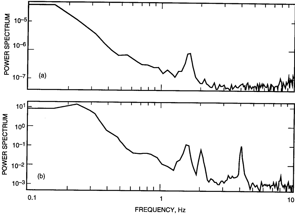
Fig. 10. Power spectra for yaw angle 180 deg and elevation angle 60 deg: (a) azimuth encoder and (b) azimuth torque.
