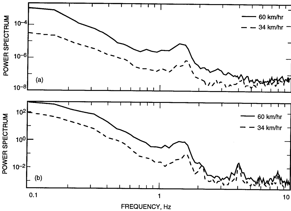
Fig. 8. Power spectra for yaw angle 180 deg and elevation angle 10 deg: (a) azimuth encoder and (b) azimuth torque.
