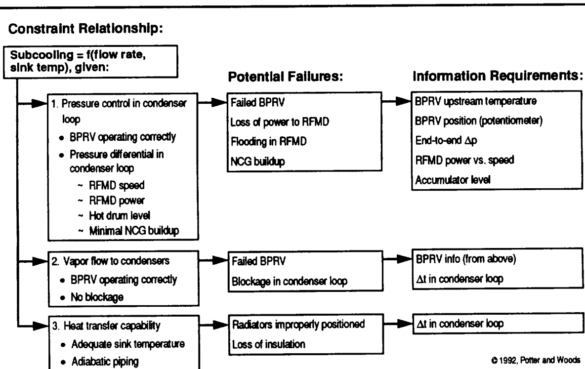
Figure 29. Relationships between functional constraints and information requirements for heat rejection.
