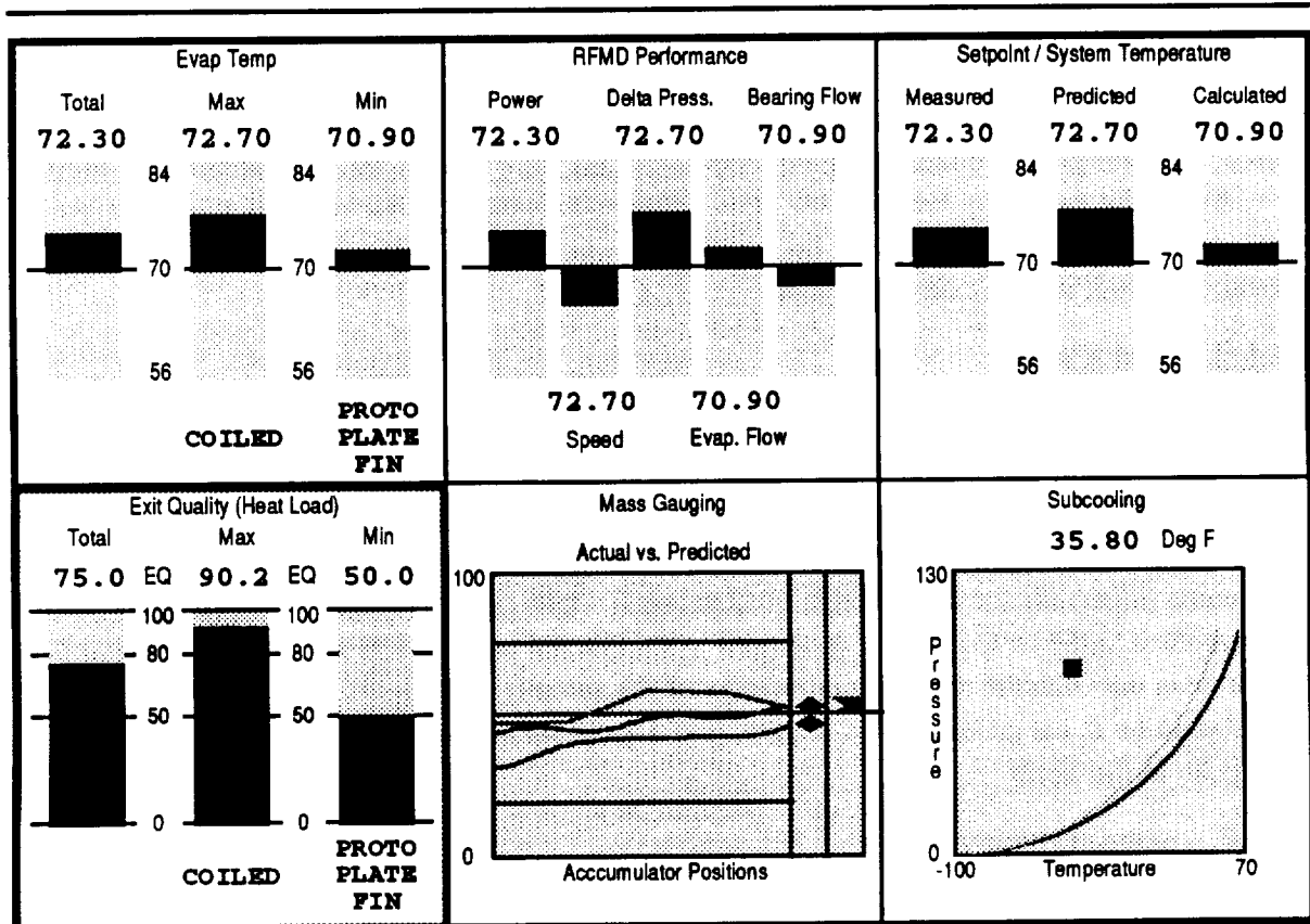
Figure 30. Function-based display for the thermal control system.
