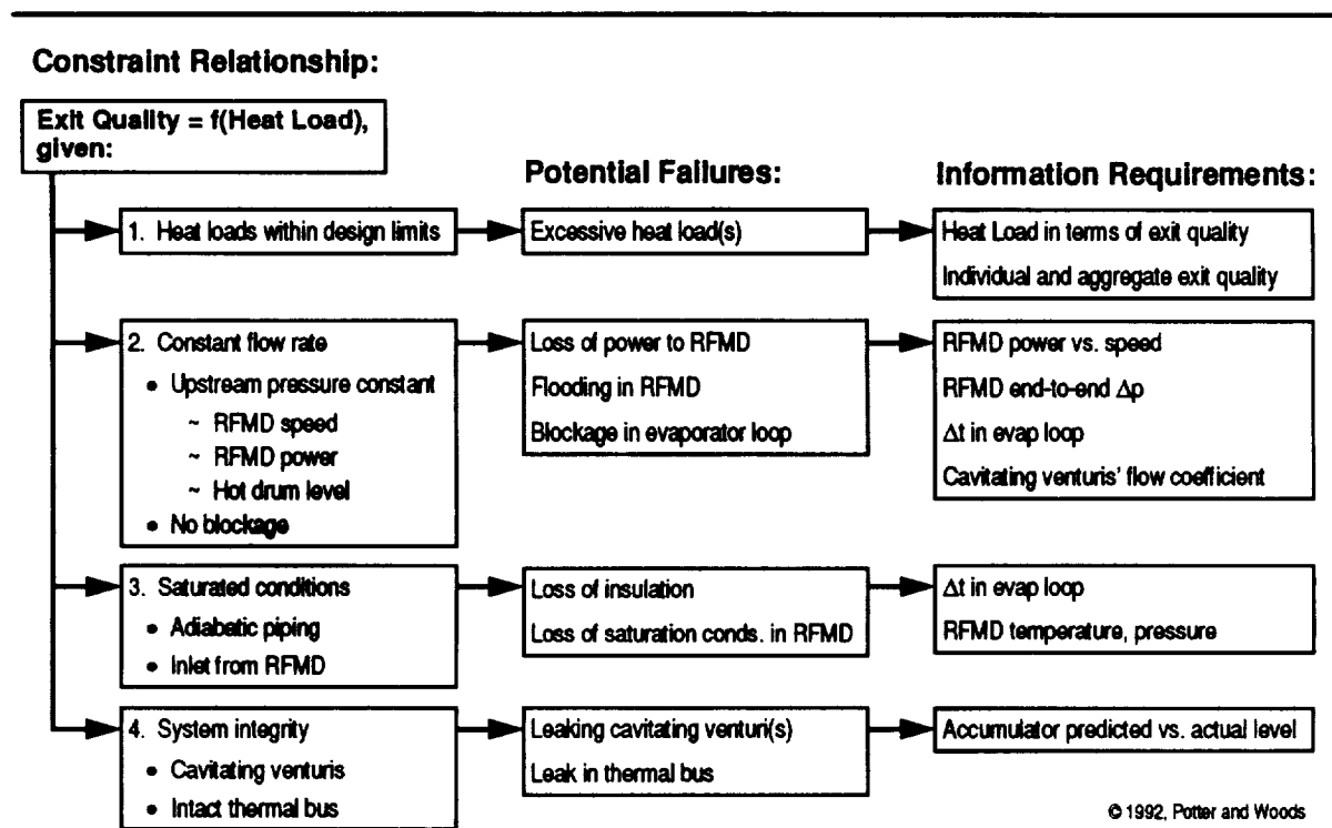
Figure 28. Relationships between functional constraints and information requirements for heat acquisition.
