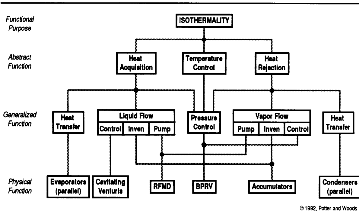
Figure 27. Functional abstraction hierarchy.
