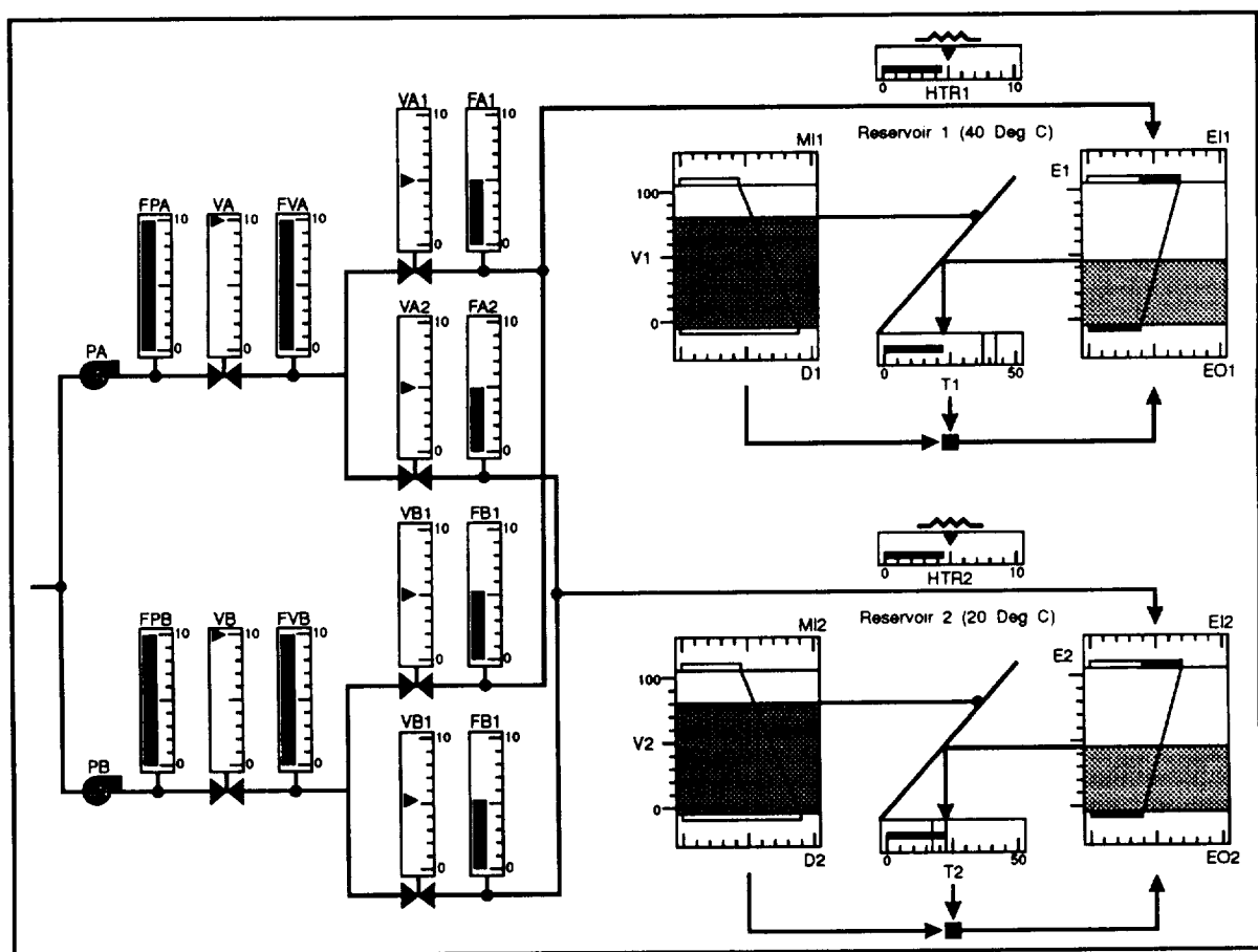
Figure 24. Functional interface for the thermal-hydraulic control system investigated by Vicente and Rasmussen (1990).
