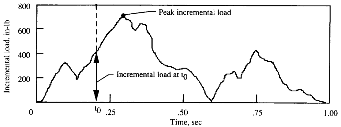
(b) Incremental load during rolling maneuver.
