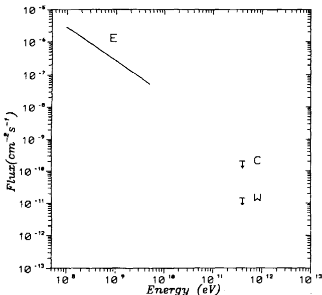
FIG. 7.—Energy spectrum for the quasar 3C 279. E: Hartman et al. (1992); C: Cawley et al. (1985); W: this paper.
