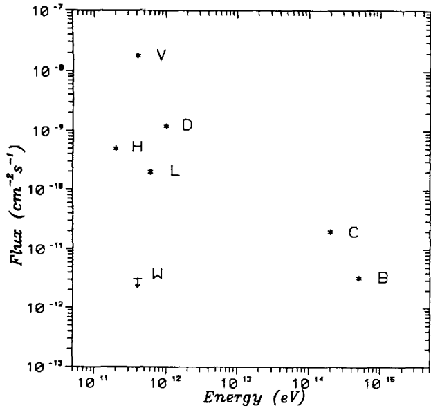
FIG. 8.—Detections and upper limits for the X-ray binary Hercules X-1. D: Douthwaite et al. (1984); B: Baltrusaitis et al. (1985); H: Resvanis et al. (1988); L: Lamb et al. (1988); C: Dingus et al. (1988); V: Vishwanath et al. (1989); W: this paper.
