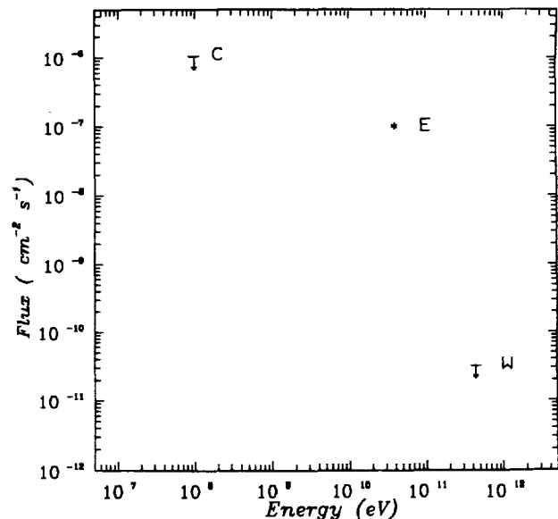
FIG. 5.—Detection and upper limits for GeV-A. C: Bignami & Hermsen (1983); E: Enomoto et al. (1990a); W: this paper.
