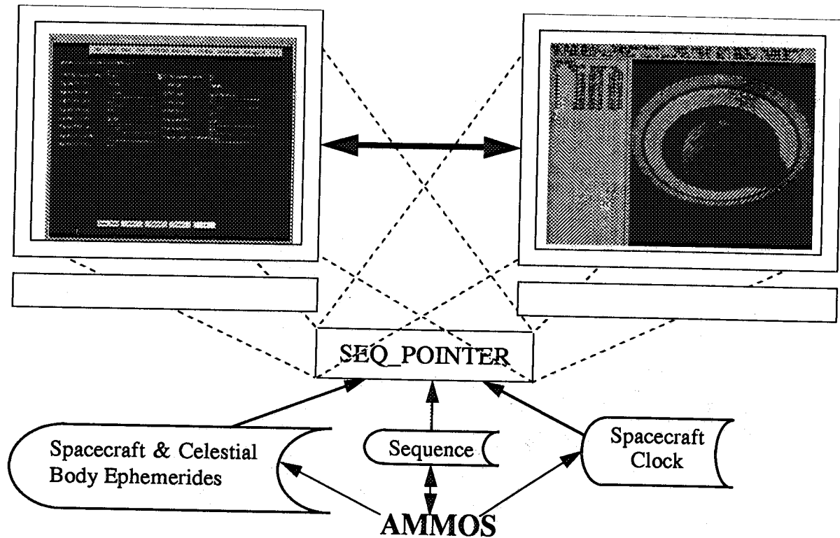
Figure 2. SEQ_POINTER in the MOSO AMMOS
