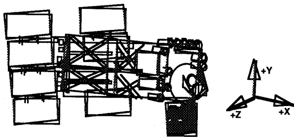
Fig. 1. MSX spacecraft
