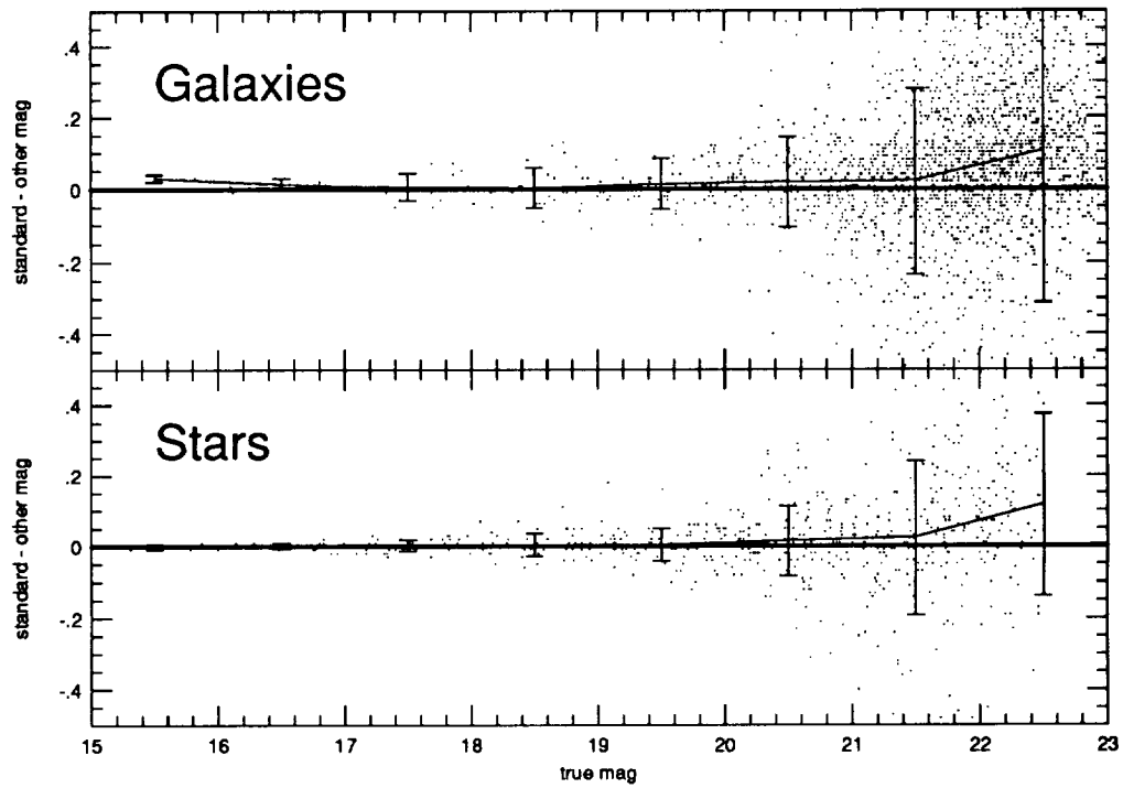
Standard ( \mu = 24.3 ) vs. Lower ( \mu = 24.5 ) Threshold
