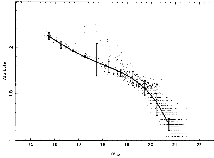
Final Fit to Stellar Locus in m_{\text{Tot}} vs. \log(\text{Area})
