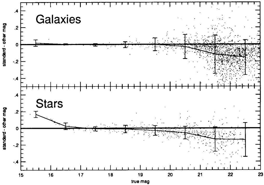
Standard 3.0" vs. 3.6" Seeing
