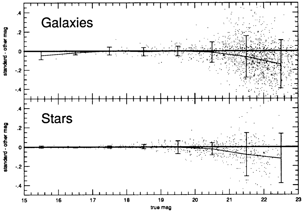
Standard ( \mu = 24.3 ) vs. Higher ( \mu = 24.1 ) Threshold
