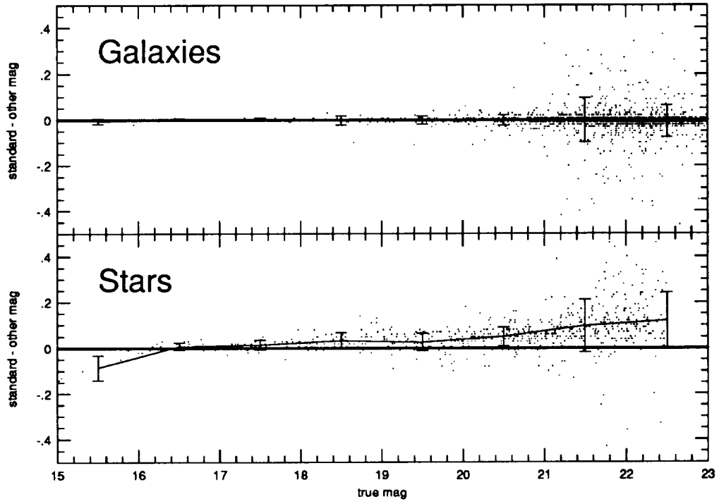
Standard Moffat (3.0") vs. Gaussian (3.0") Seeing
