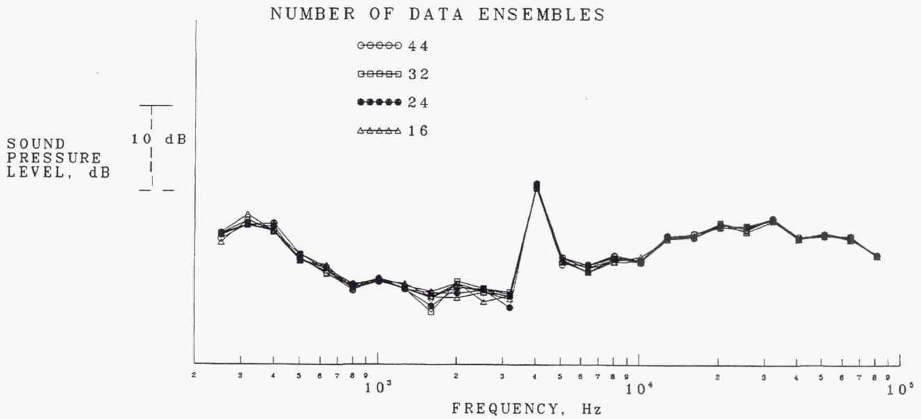
Figure 16.—Repeat 1/3rd octave SPL spectra for model turbfan showing effect of number of data ensembles (fixed wall microphone, 0.20 M).
