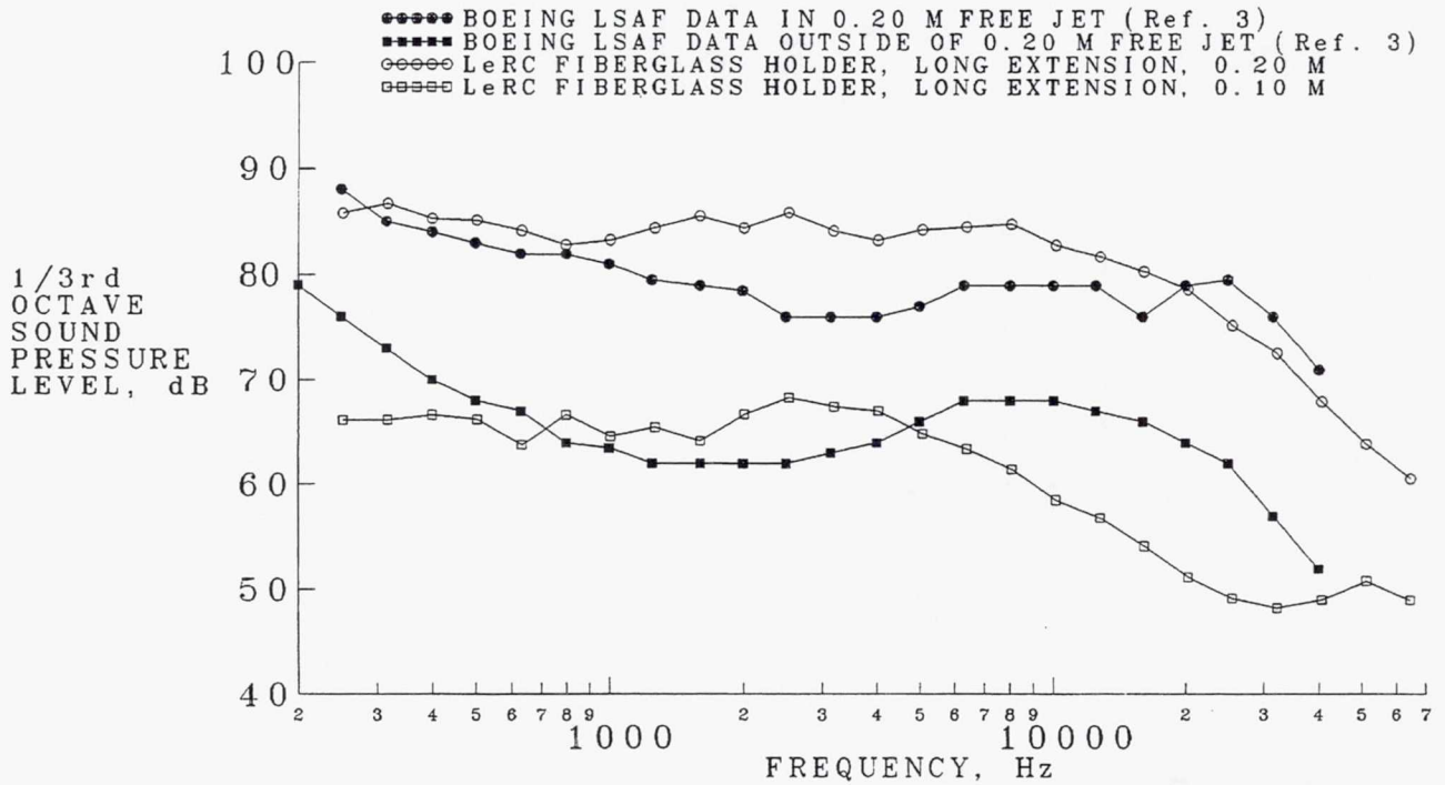
Figure 8.—Reductions in tunnel background noise levels with reduced tunnel velocity (wall mount, Ames-profile fiberglass holder).
