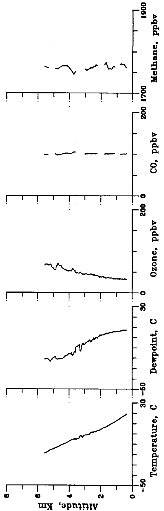
ABLE-3B CANADIAN MISSION: FLIGHT 2 PROFILE AT 2200 GMT
