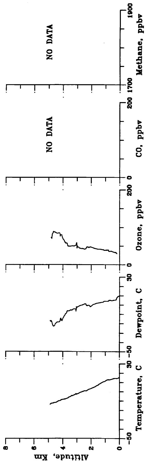
ABLE-3A ALASKAN MISSION: FLIGHT 31 PROFILE AT 2045 GMT
