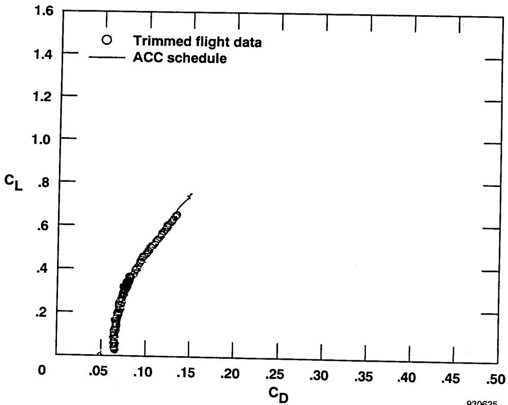
(i) M = 1.20 . (Note: Units for \alpha , above, are degrees.)
