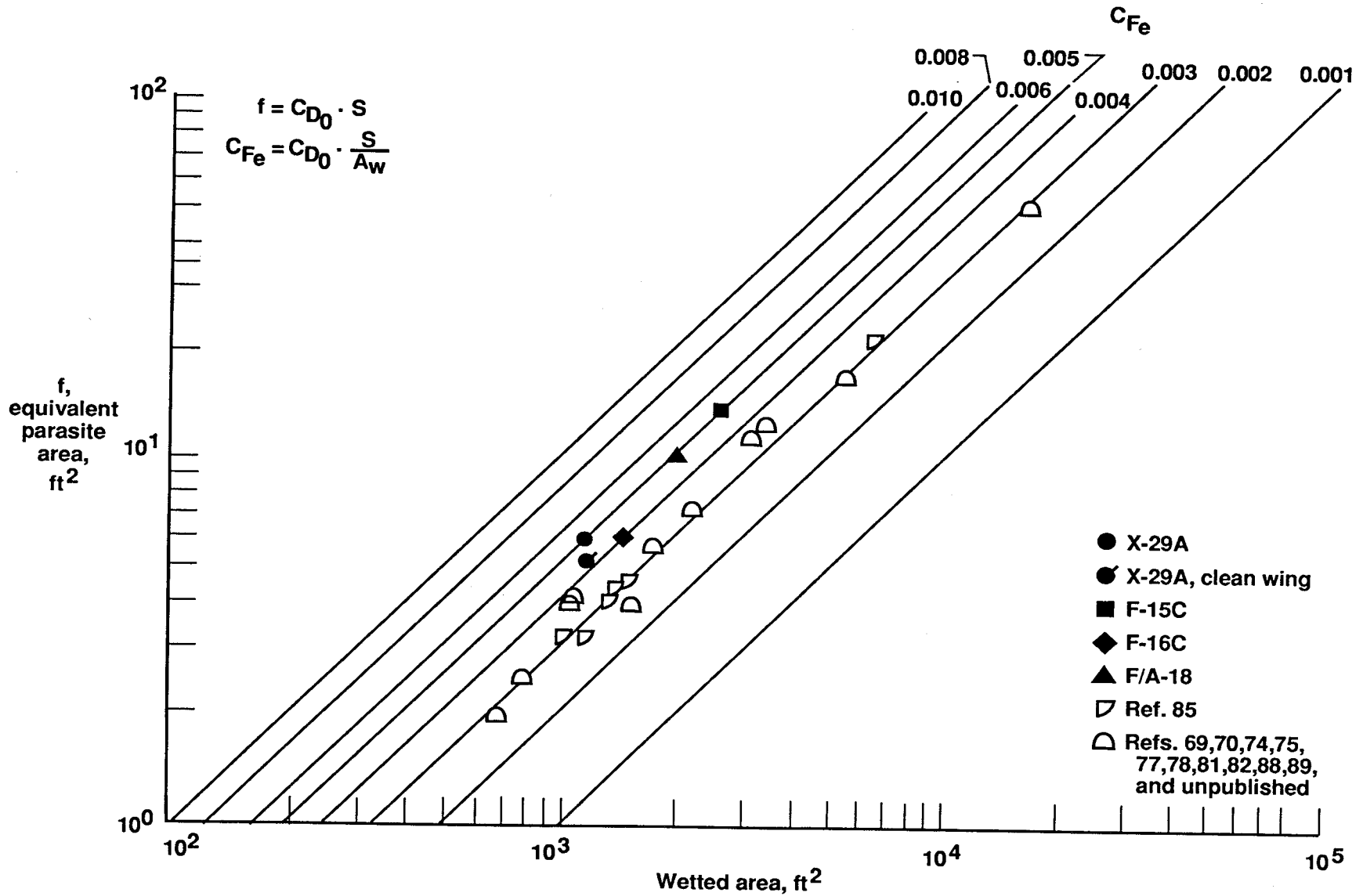
Figure 30. Relationship of equivalent parasite area and C_{f_e} to total wetted area for several aircraft at subsonic Mach numbers; flight data.
