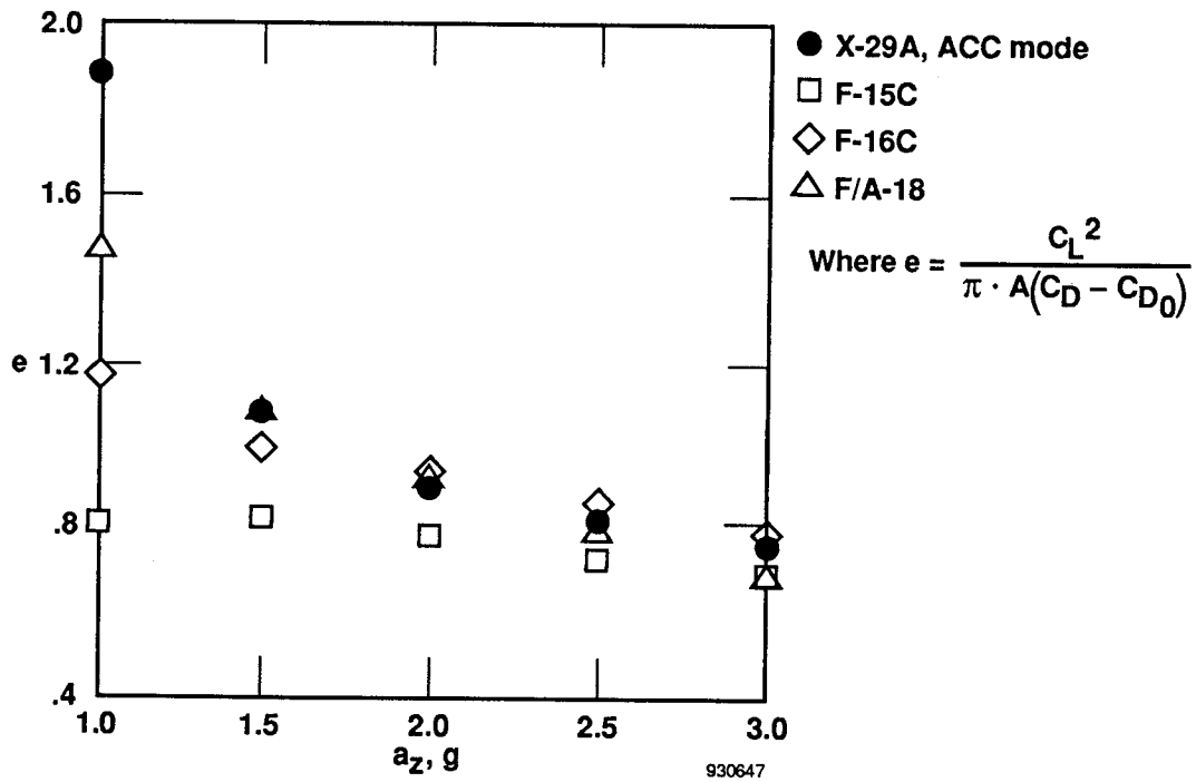
(a) Asymmetric polars for X-29A, F/A-18, and F-16C.
