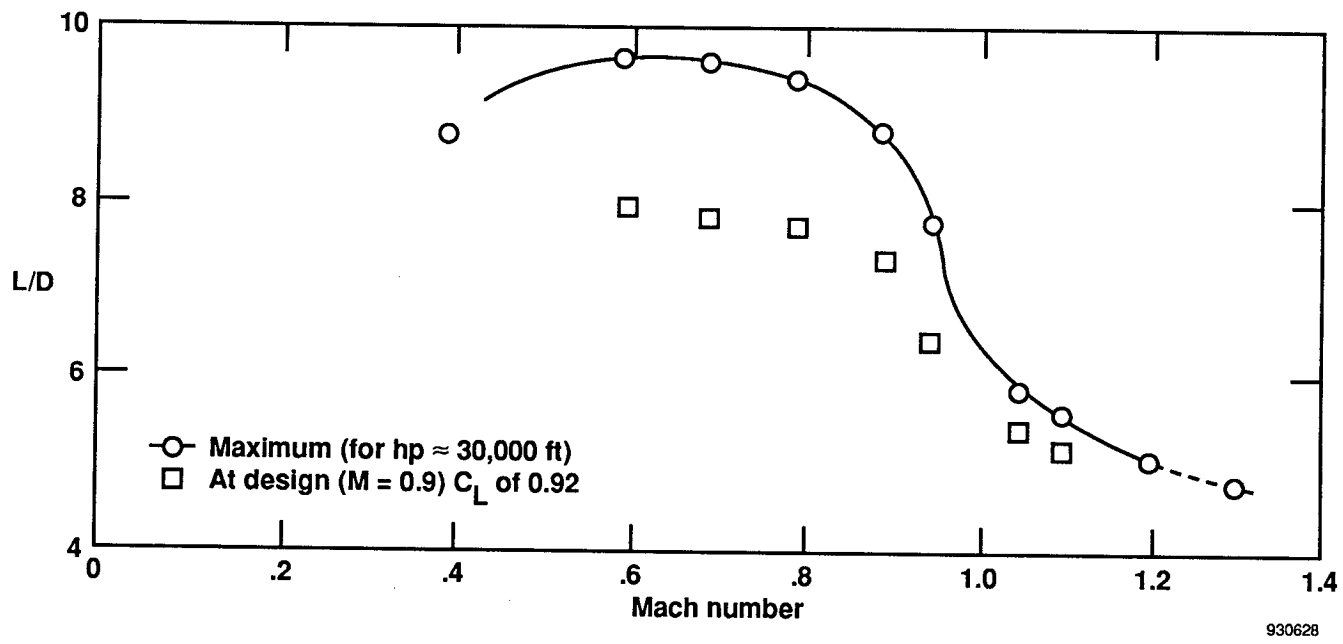
Figure 8. Variation of lift-drag ratio with Mach number; trimmed flight, ACC control mode.
