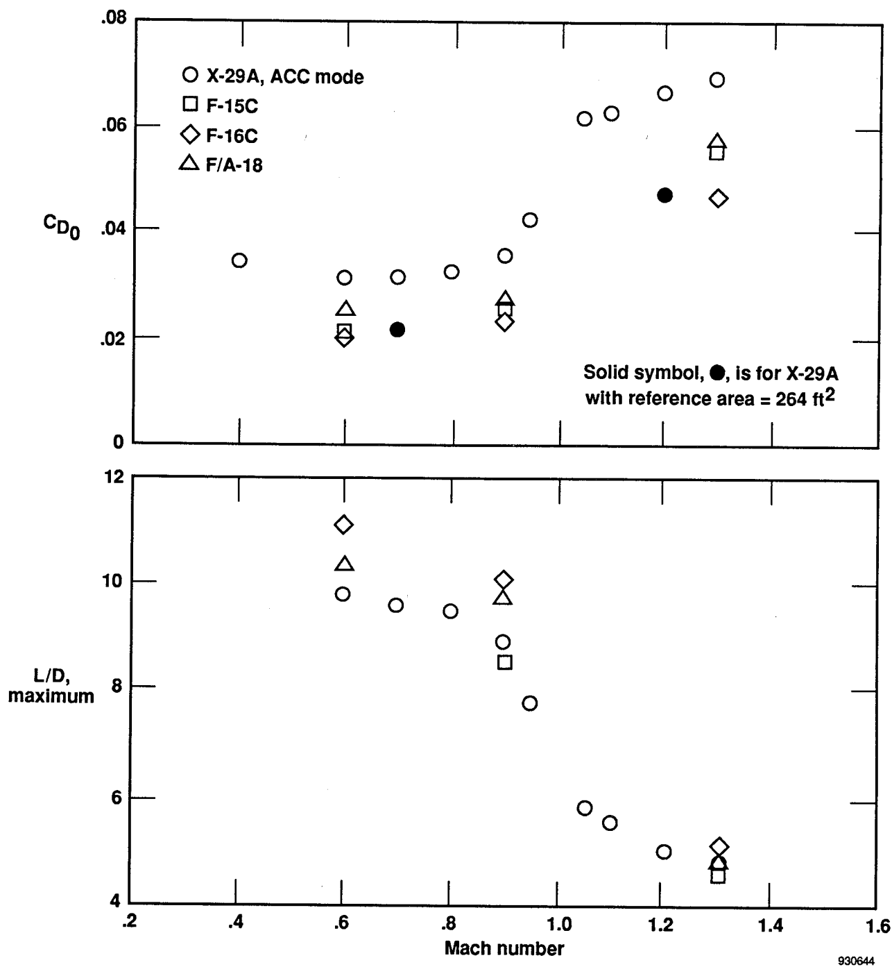
Figure 23. Variation of zero-lift-drag coefficient and maximum L/D with Mach number for X-29A and three contemporary aircraft.
