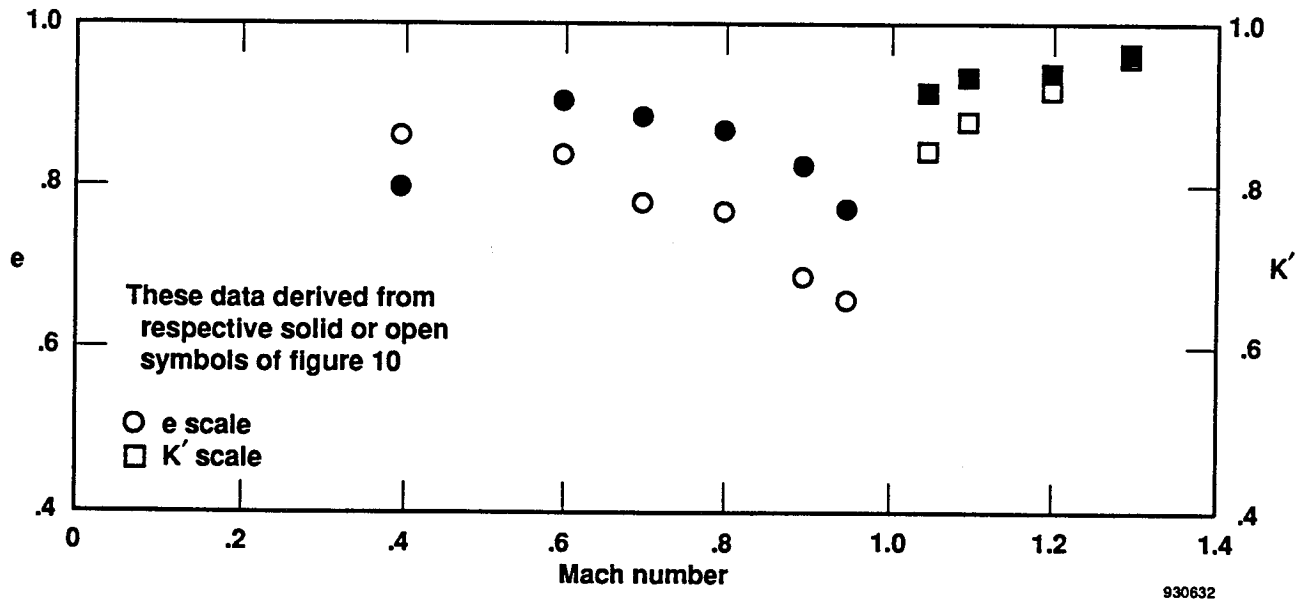
Figure 12. Variation of airplane lifting efficiency factors, e and K' , with Mach number; trimmed flight, ACC mode.
