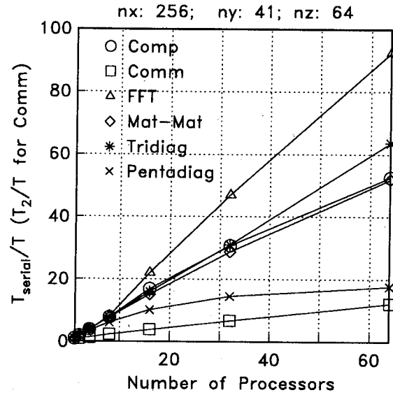
(b) speedup.
