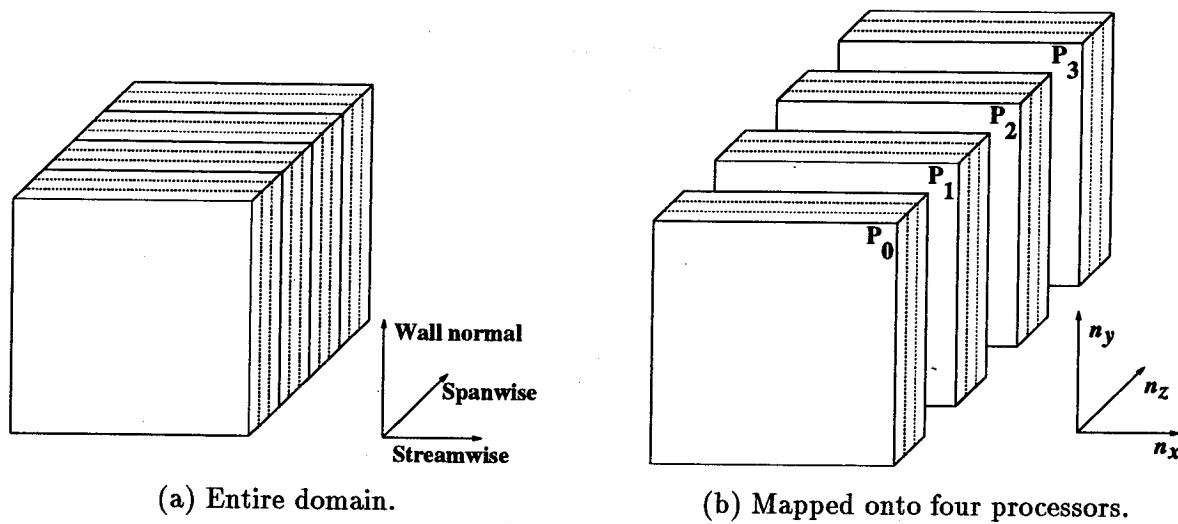
Figure 1: Computational domain.
