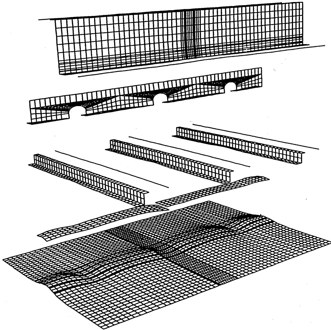
Figure 5: Exploded deformed view of the intermediate model of 1 x 3 bays of fuselage panel.
