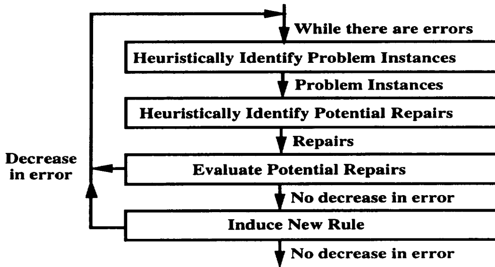
Figure 1: System Organization.
