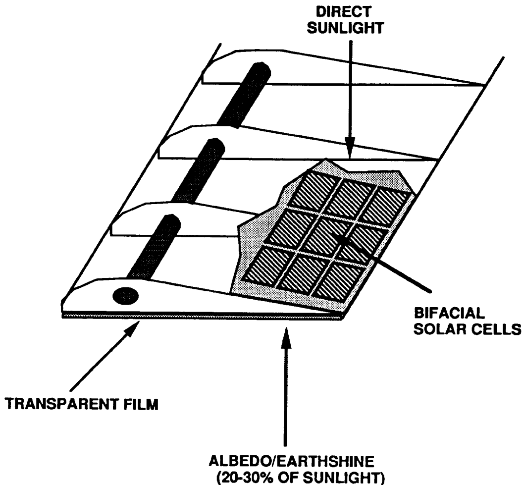
Fig. 6: UAV Wing Construction Can Support Bifacial Solar Cell Insolation
